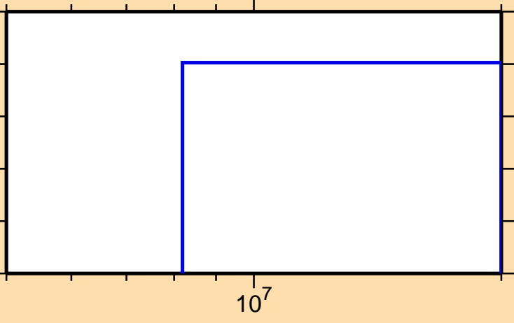
\sigma vs. E for ^{194}\text{Ir}(n,nt)
