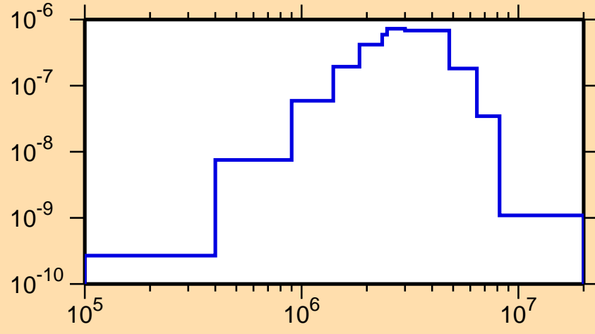
\sigma vs. E for ^{194}\text{Ir}(n,n_1)
