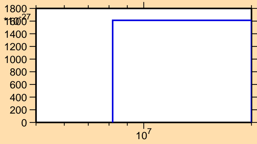
\sigma vs. E for ^{196}\text{Ir}(\text{mt } 42)
