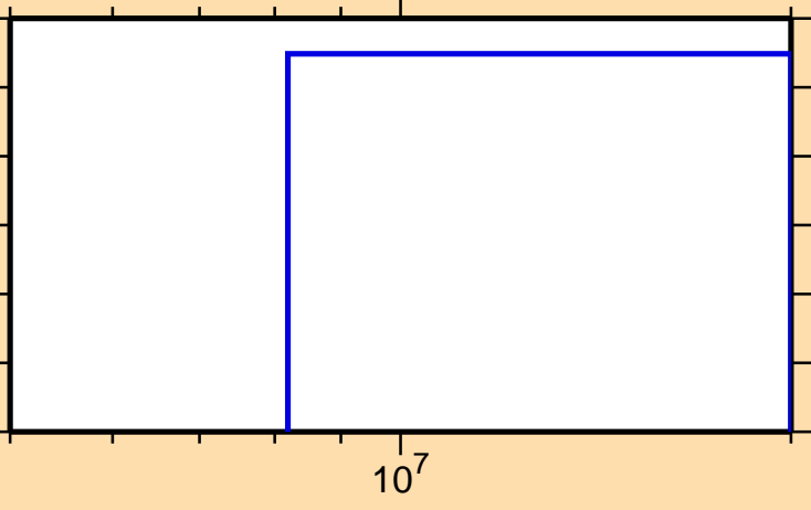
\sigma vs. E for ^{196}\text{Ir}(n,nt)
