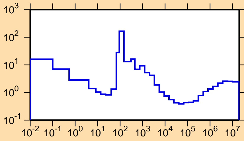
\sigma vs. E for ^{197}\text{Ir}(n,\text{nonel.})
