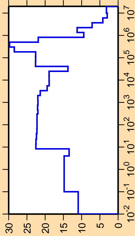
\Delta\sigma/\sigma vs. E for ^{197}\text{Ir}(n,\text{nonel.})
