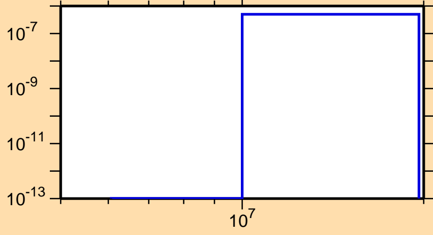
\sigma vs. E for ^{197}\text{Ir}(n,n\alpha)
