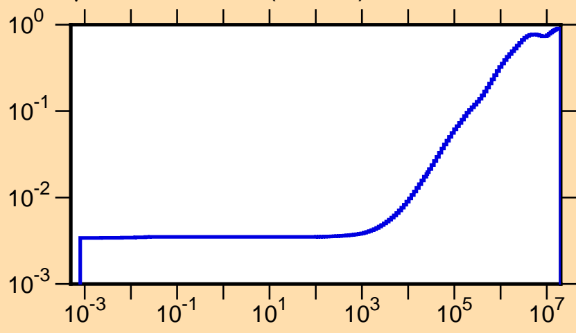
\mu vs. E for ^{198}\text{Ir}(\text{mt251})
