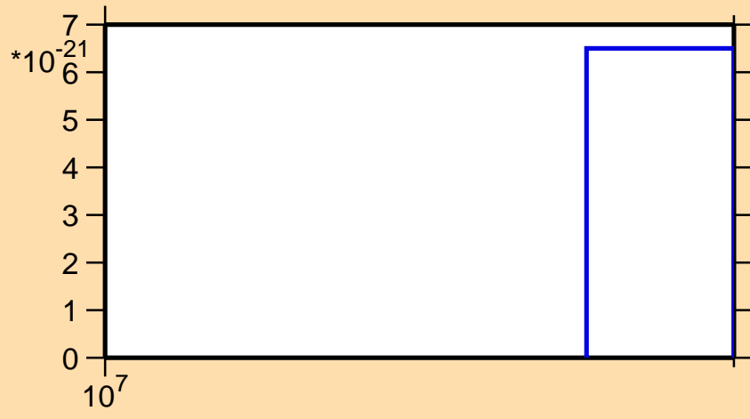
\sigma vs. E for ^{198}\text{Ir} (mt 42)
