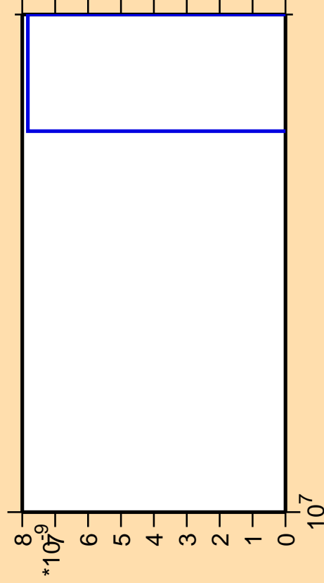
\Delta\sigma/\sigma vs. E for ^{198}\text{Ir} (mt 42)
