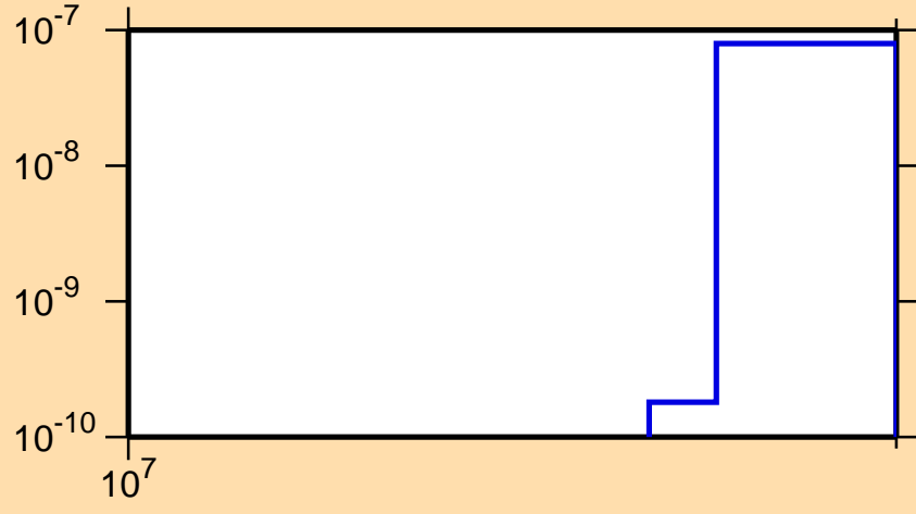
\sigma vs. E for ^{198}\text{Ir}(n,2np)
