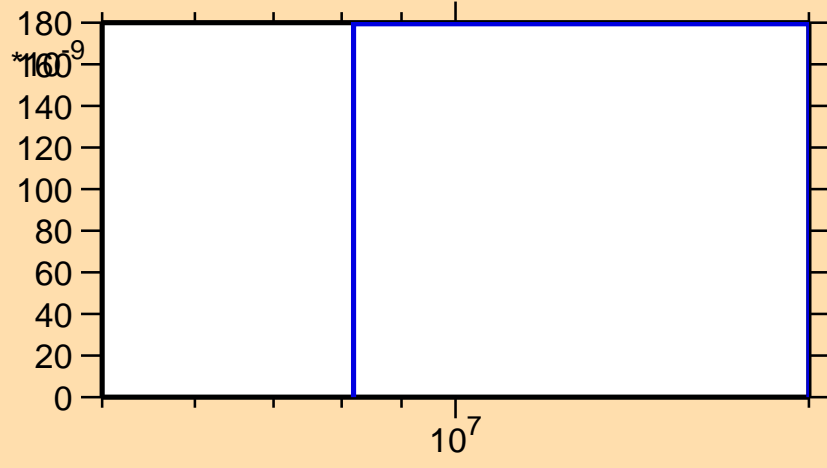
\sigma vs. E for ^{198}\text{Ir}(n,n\alpha)
