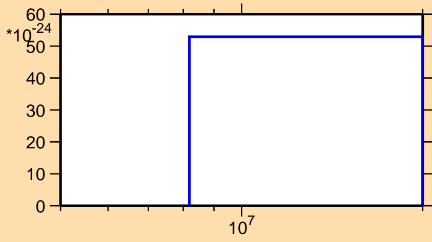
\sigma vs. E for ^{198}\text{Ir}(\text{mt } 42)
