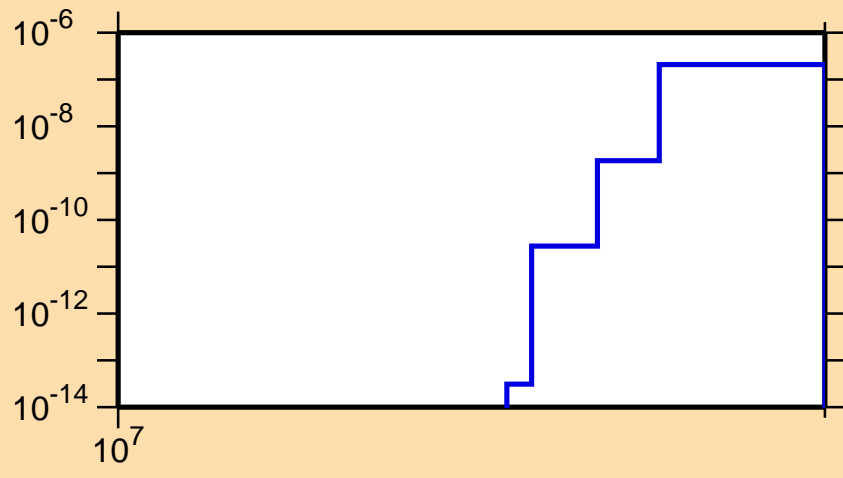
\sigma vs. E for ^{199}\text{Ir}(n,nt)
