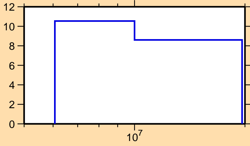
\Delta\sigma/\sigma vs. E for ^{201}\text{Ir}(n,\text{nonel.})
