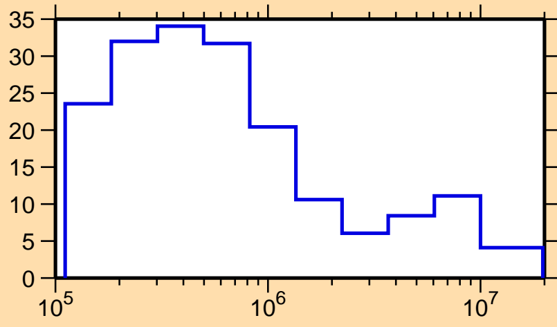
\Delta\sigma/\sigma vs. E for ^{201}\text{Ir}(n,\text{tot.})
