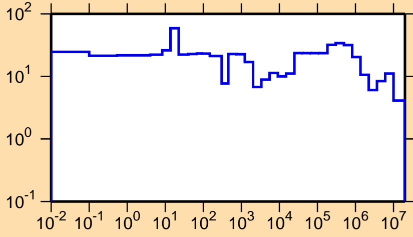
\Delta\sigma/\sigma vs. E for ^{201}\text{Ir}(n,\text{tot.})
