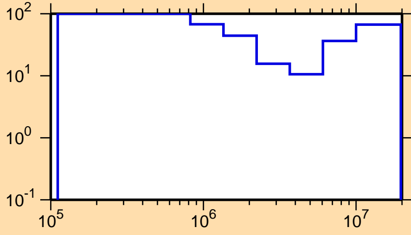
\Delta\sigma/\sigma vs. E for ^{201}\text{Ir}(n,n\text{cont.})
