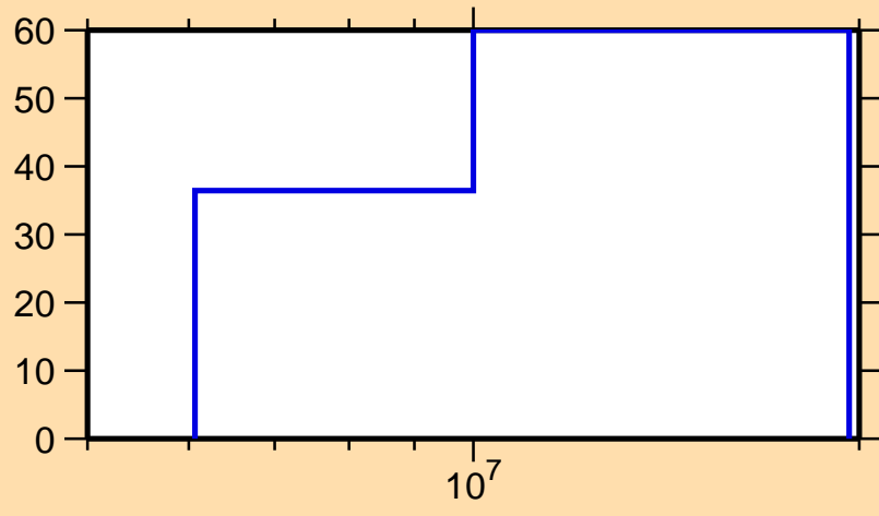
\Delta\sigma/\sigma vs. E for ^{201}\text{Ir}(n,n\text{cont.})
