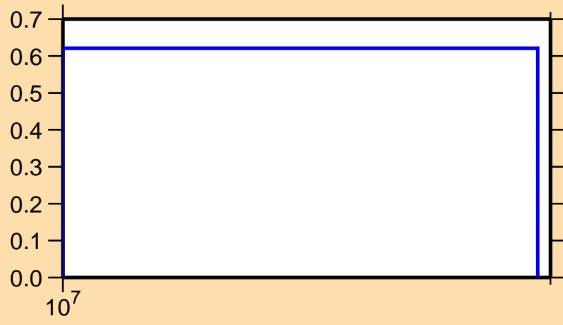
\sigma vs. E for ^{201}\text{Ir}(n,3n)
