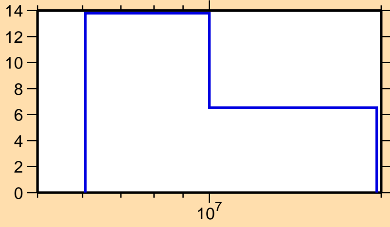
\Delta\sigma/\sigma vs. E for ^{201}\text{Ir}(n,\text{el.})
