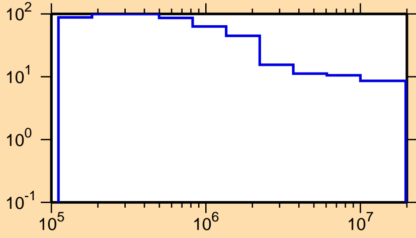
\Delta\sigma/\sigma vs. E for ^{201}\text{Ir}(n,\text{nonel.})
