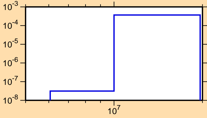
\sigma vs. E for ^{201}\text{Ir}(n,p)
