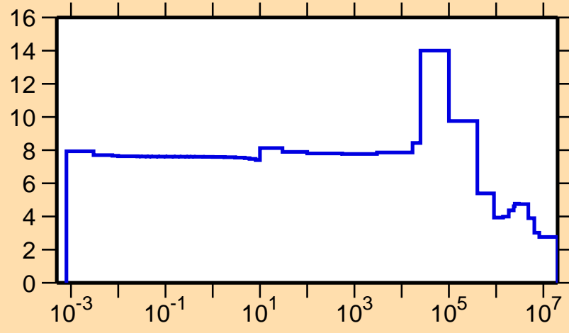
\sigma vs. E for ^{201}\text{Ir}(n,\text{el.})
