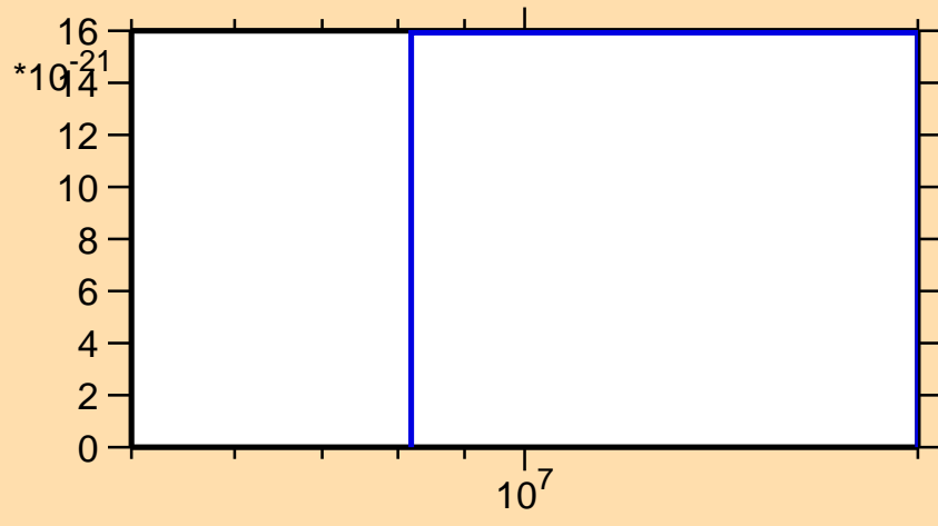
\sigma vs. E for ^{201}\text{Ir}(\text{mt } 42)
