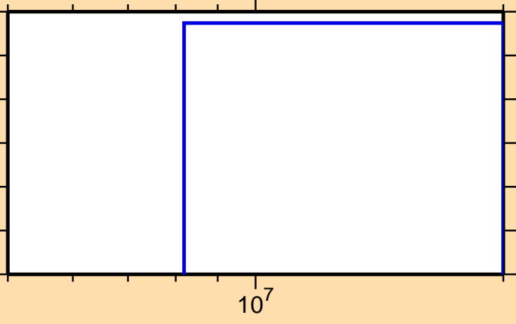
\sigma vs. E for ^{201}\text{Ir}(n,np)
