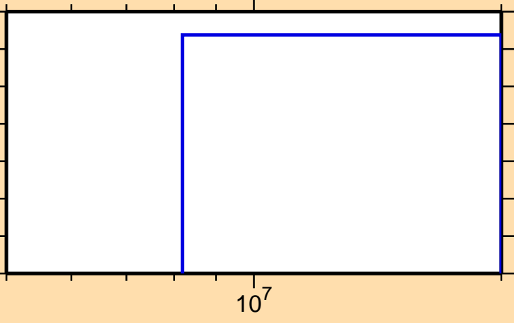
\sigma vs. E for ^{201}\text{Ir}(n,d)
