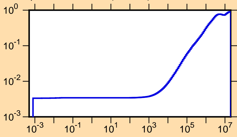
\mu vs. E for ^{202}\text{Ir}(\text{mt251})
