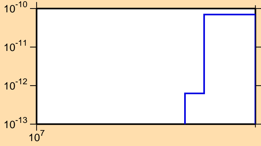
\sigma vs. E for ^{202}\text{Ir}(n,2n\alpha)
