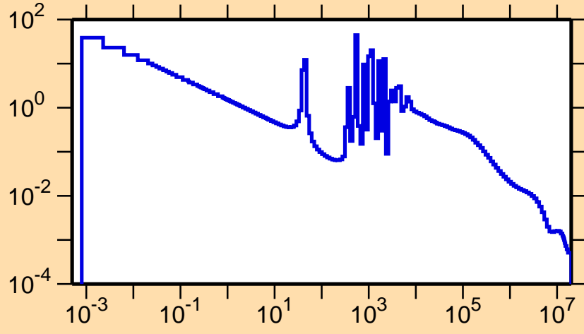
\sigma vs. E for ^{202}\text{Ir}(n,\gamma)
