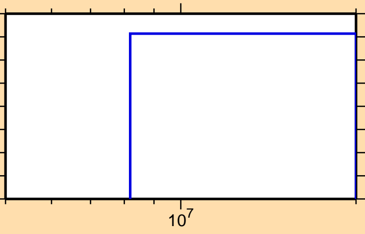
\sigma vs. E for ^{202}\text{Ir}(n,np)
