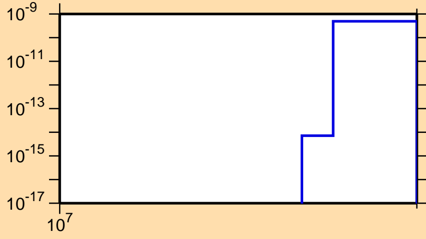
\sigma vs. E for ^{203}\text{Ir}(n,2np)
