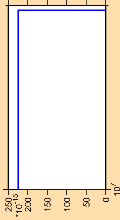
\Delta\sigma/\sigma vs. E for ^{203}\text{Ir} (mt 42)
