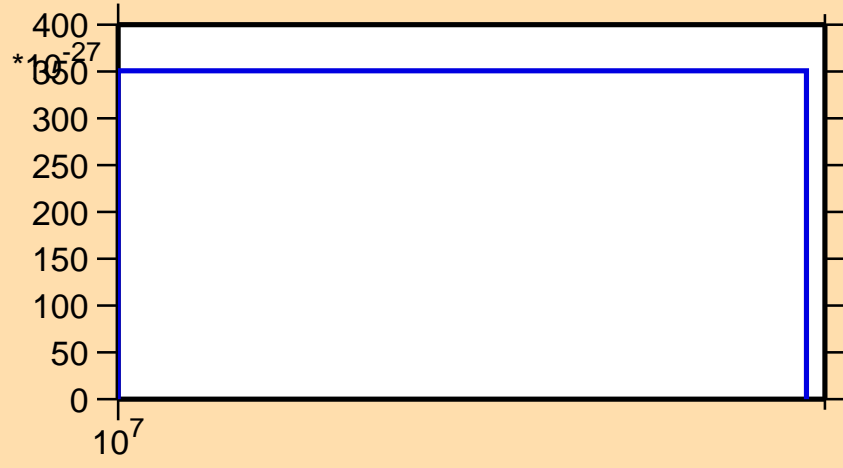
\sigma vs. E for ^{203}\text{Ir} (mt 42)
