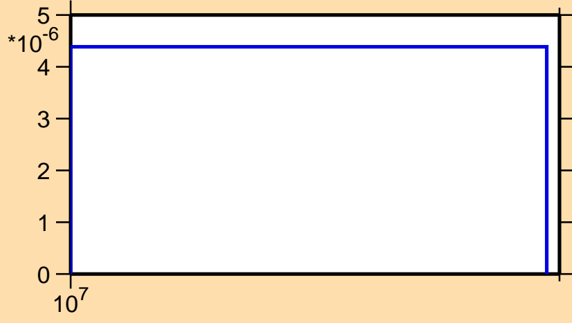
\sigma vs. E for ^{203}\text{Ir}(n,np)
