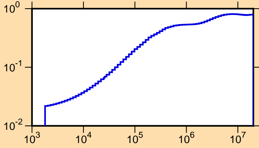
\mu vs. E for ^{37}\text{K}(\text{mt251})
