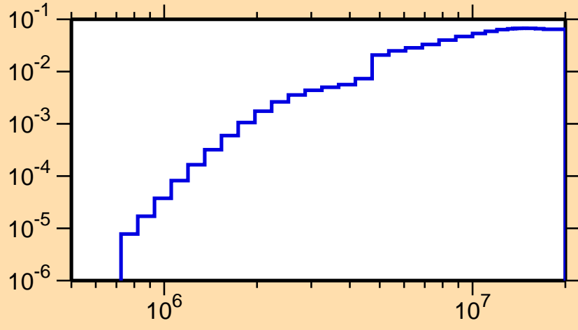
\sigma vs. E for ^{37}\text{K}(n,d)
