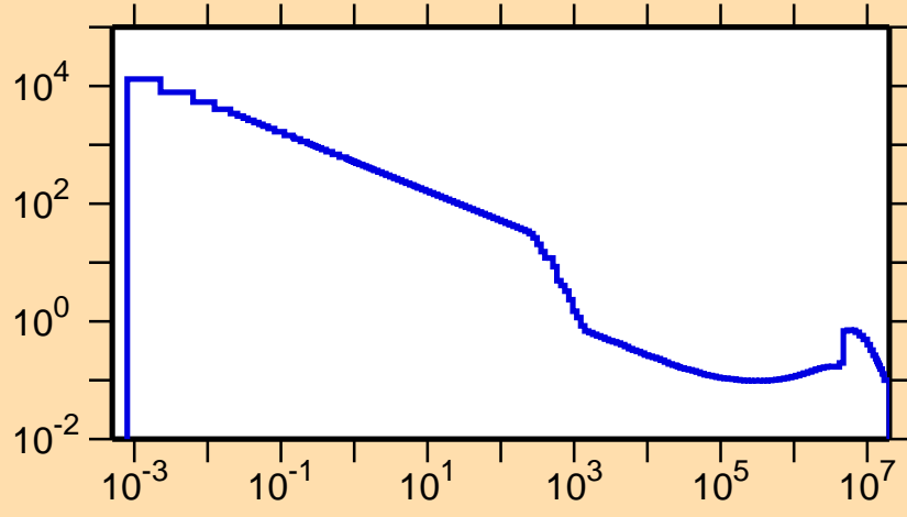
\sigma vs. E for ^{37}\text{K}(n,\alpha)
