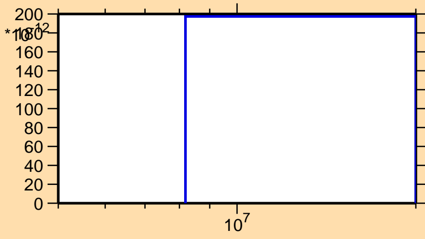
\sigma vs. E for ^{37}\text{K}(\text{mt } 34)
