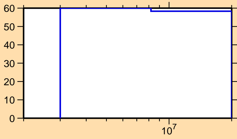
\Delta\sigma/\sigma vs. E for ^{37}\text{K}(n,ncont.)
