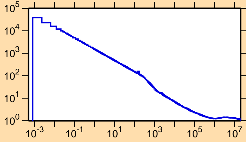
\sigma vs. E for ^{38}\text{K}(n,\text{nonel.})
