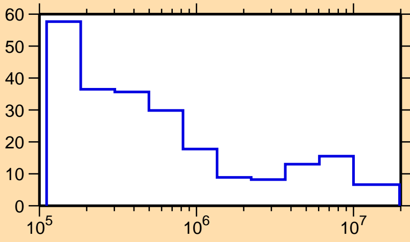
\Delta\sigma/\sigma vs. E for ^{38}\text{K}(n,\text{el.})
