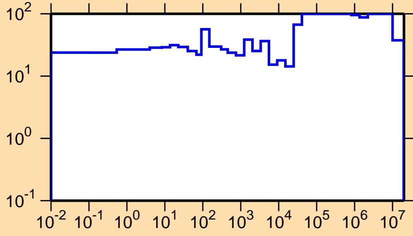
\Delta\sigma/\sigma vs. E for ^{38}\text{K}(n,\gamma)
