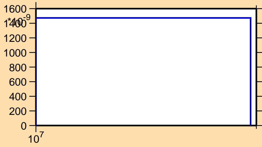
\sigma vs. E for ^{38}\text{K} (mt 45)
