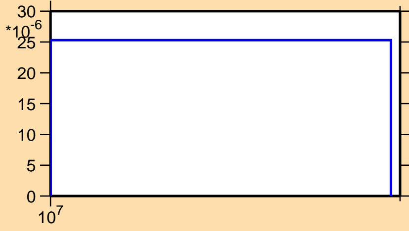
\sigma vs. E for ^{38}\text{K}(n,pd)
