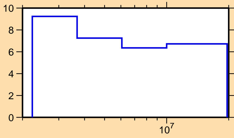
\Delta\sigma/\sigma vs. E for ^{38}\text{K}(n,n\text{onel.})
