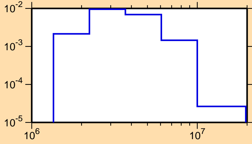
\sigma vs. E for ^{38}\text{K}(n,n_3)
