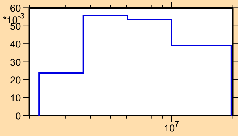
\sigma vs. E for ^{38}\text{K}(n,n_4)
