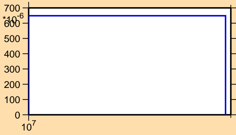
\sigma vs. E for ^{38}\text{K}(n,2n)
