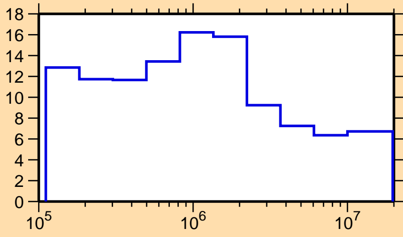
\Delta\sigma/\sigma vs. E for ^{38}\text{K}(n,\text{nonel.})
