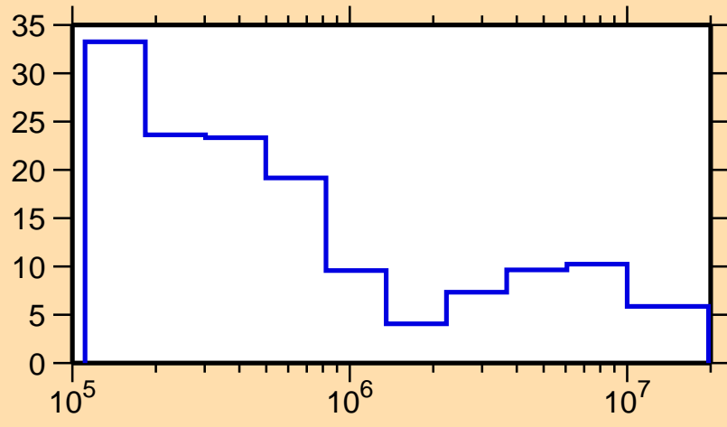
\Delta\sigma/\sigma vs. E for ^{38}\text{K}(n,\text{tot.})
