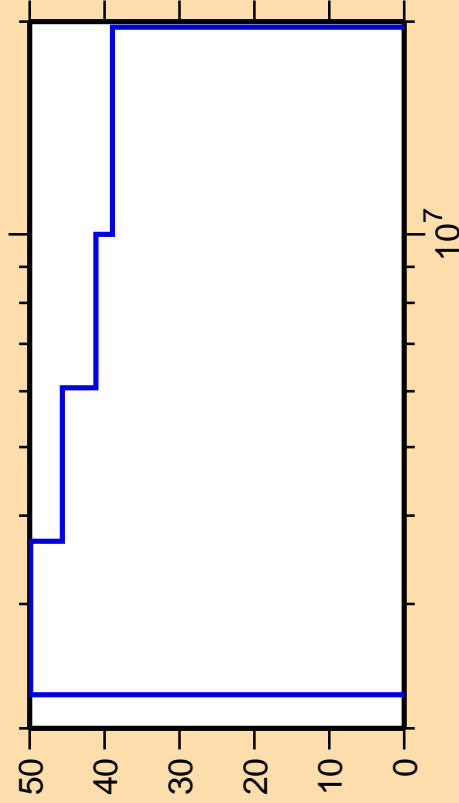
\Delta\sigma/\sigma vs. E for ^{38}\text{K}(n,n_4)
