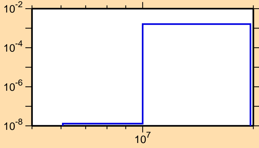
\sigma vs. E for ^{38}\text{K}(n,\text{He}3)
