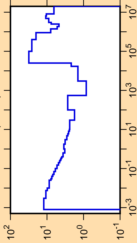
\Delta\sigma/\sigma vs. E for ^{38}\text{K}(n,\text{tot.})
