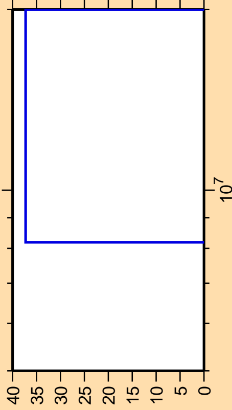
\Delta\sigma/\sigma vs. E for ^{38}\text{K}(n,p)
