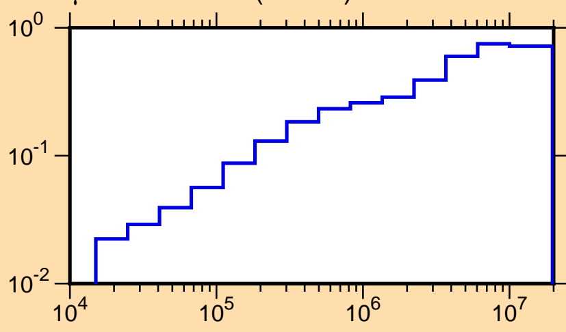
\mu vs. E for ^{39}\text{K}(\text{mt251})
