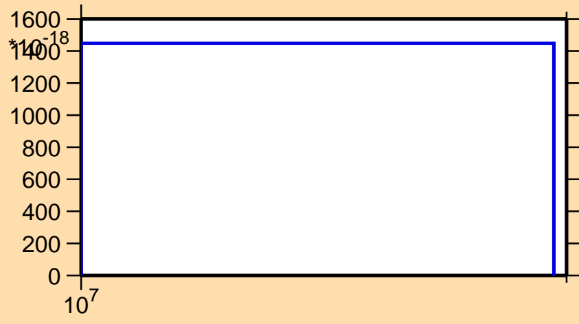
\sigma vs. E for ^{39}\text{K}(n,nt)
