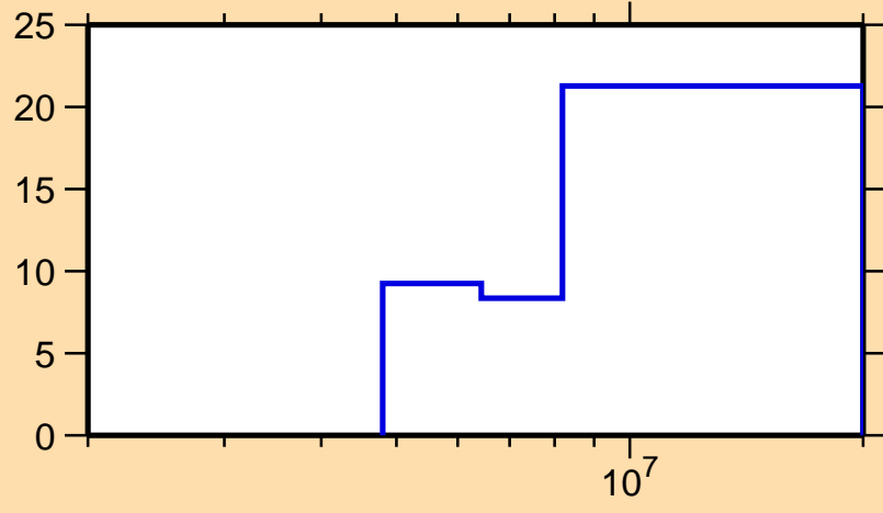
\Delta\sigma/\sigma vs. E for ^{39}\text{K}(n,inel.)
