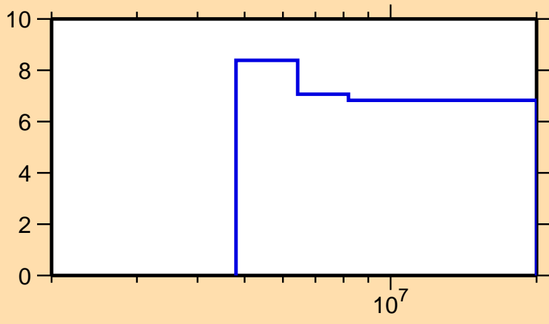
\Delta\sigma/\sigma vs. E for ^{39}\text{K}(n,n\text{onel.})
