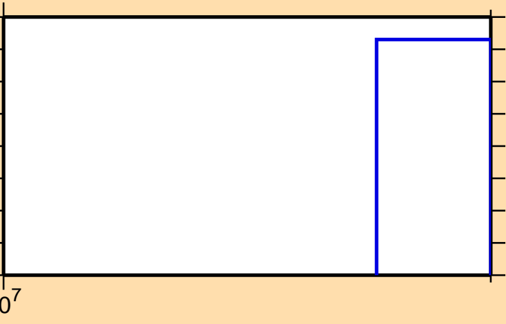
\sigma vs. E for ^{40}\text{K}(n,nt)
