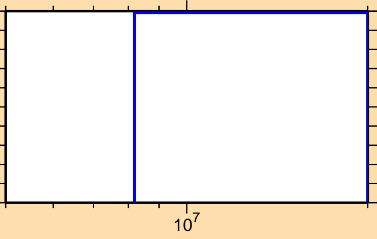
\sigma vs. E for ^{40}\text{K}(n,2n\alpha)
