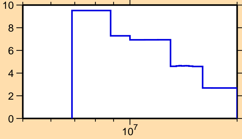
\Delta\sigma/\sigma vs. E for ^{42}\text{K}(n,\text{tot.})
