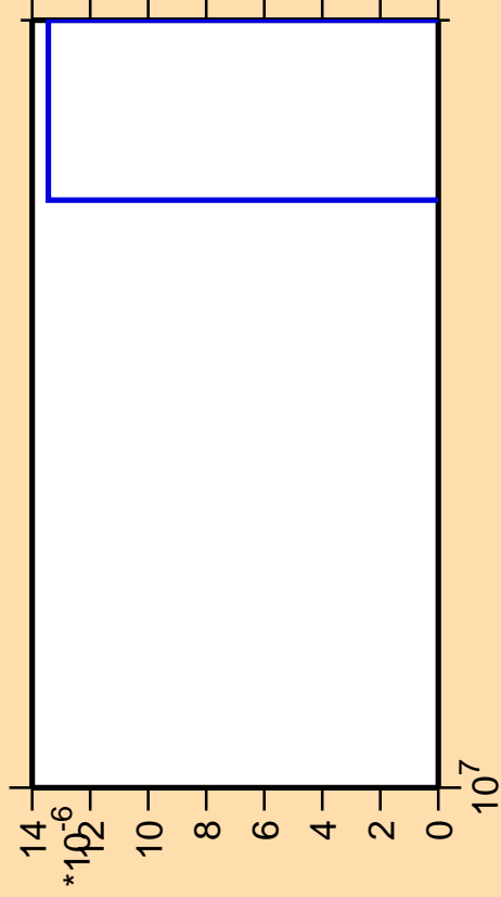
\Delta\sigma/\sigma vs. E for ^{42}\text{K} (mt 45)
