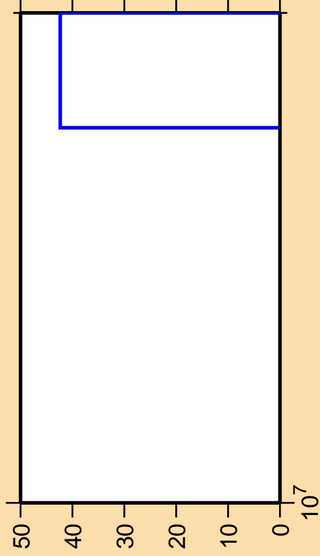
\Delta\sigma/\sigma vs. E for ^{42}\text{K}(n,3n)
