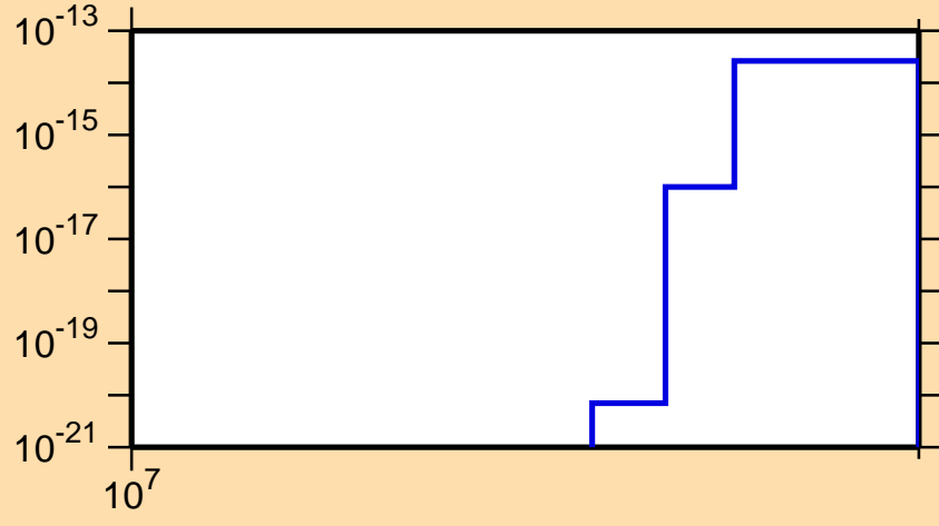
\sigma vs. E for ^{42}\text{K}(\text{mt117})
