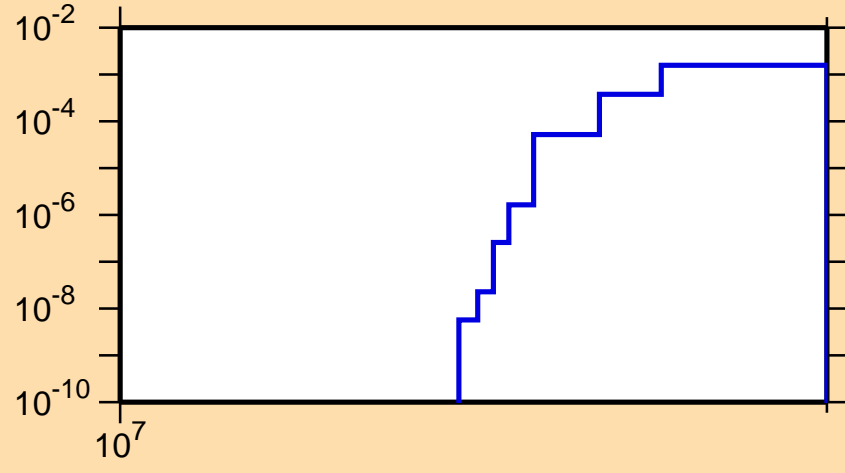
\sigma vs. E for ^{42}\text{K}(n,nd)
