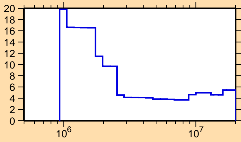
\Delta\sigma/\sigma vs. E for ^{42}\text{K}(n,\text{nonel.})
