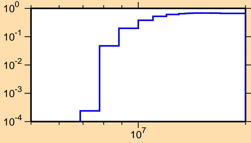
\sigma vs. E for ^{42}\text{K}(n,2n)
