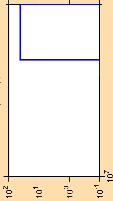
\Delta\sigma/\sigma vs. E for ^{42}\text{K}(n,2np)
