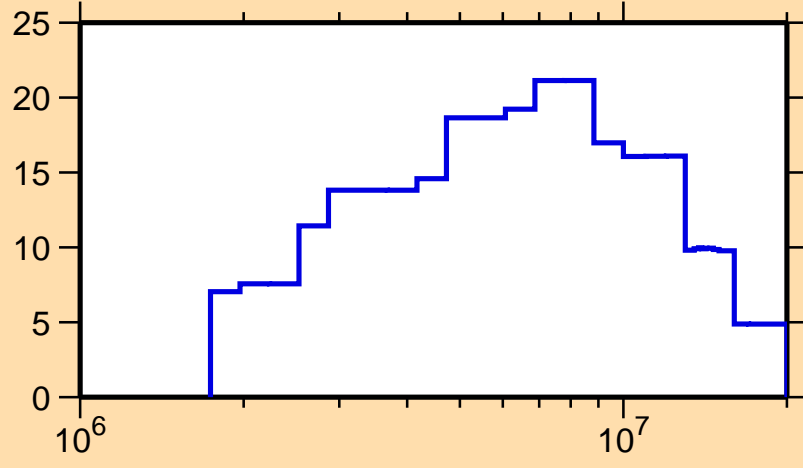
\Delta\sigma/\sigma vs. E for ^{42}\text{K}(n,el.)
