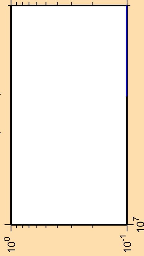
\Delta\sigma/\sigma vs. E for ^{42}\text{K}(\text{mt117})
