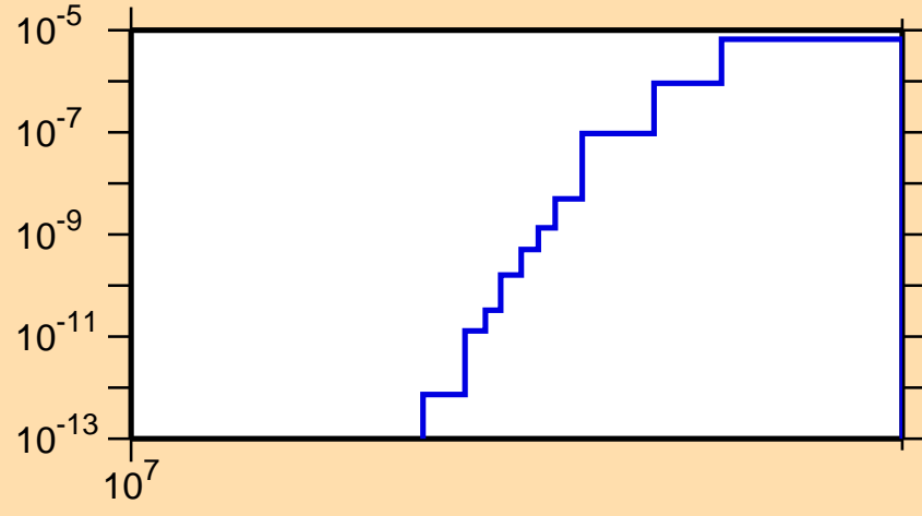
\sigma vs. E for ^{42}\text{K}(n,p\alpha)
