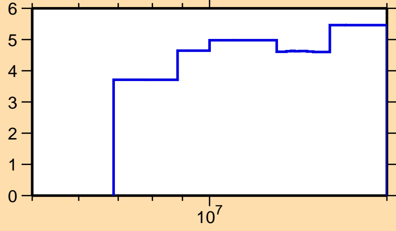
\Delta\sigma/\sigma vs. E for ^{42}\text{K}(n,\text{nonel.})
