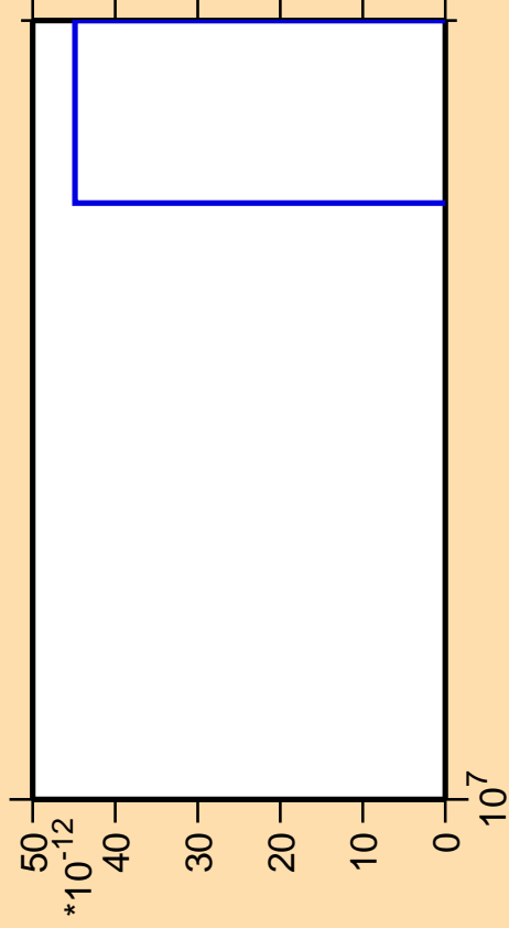
\Delta\sigma/\sigma vs. E for ^{42}\text{K}(n,pt)
