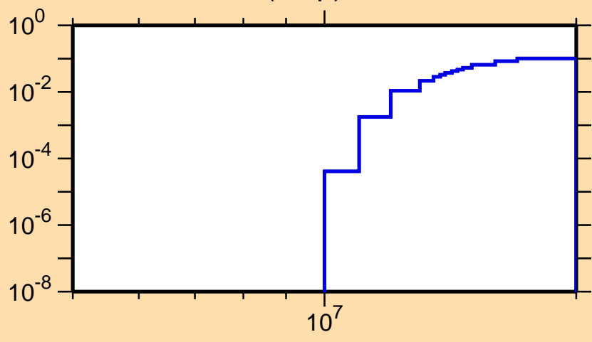
\sigma vs. E for ^{42}\text{K}(n,np)
