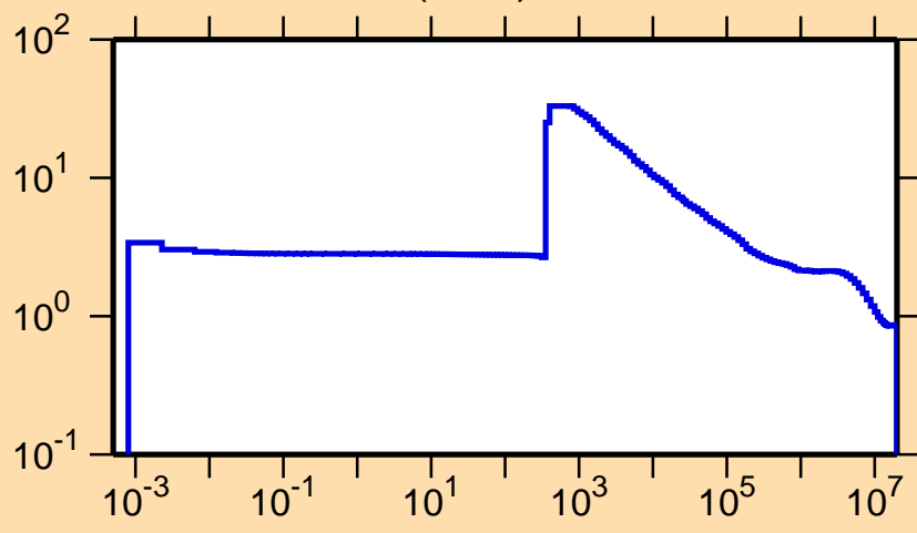
\sigma vs. E for ^{42}\text{K}(n,\text{el.})
