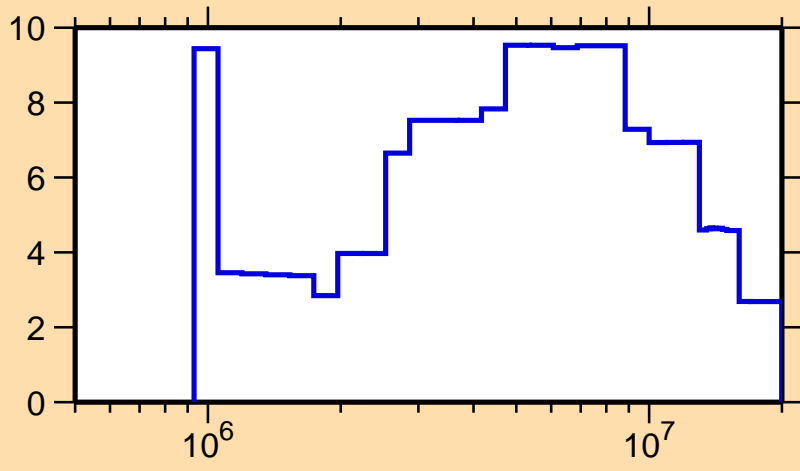
\Delta\sigma/\sigma vs. E for ^{42}\text{K}(n,\text{tot.})
