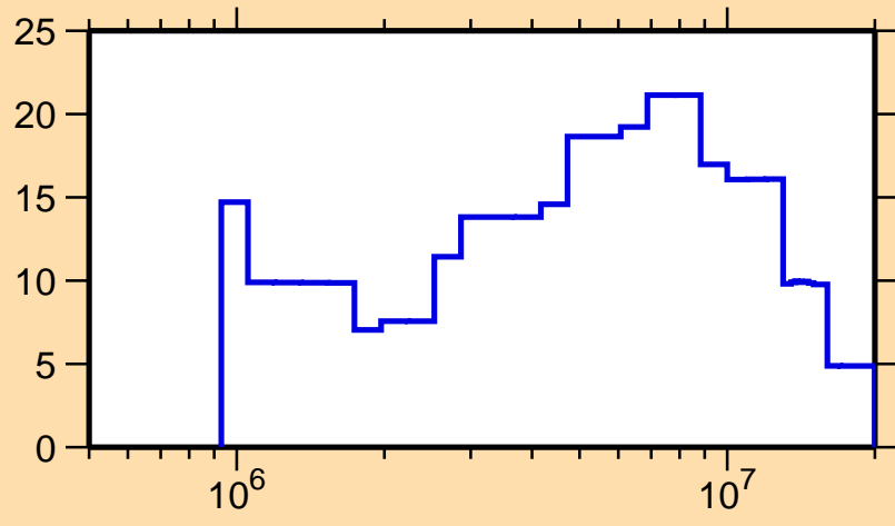
\Delta\sigma/\sigma vs. E for ^{42}\text{K}(n,\text{el.})
