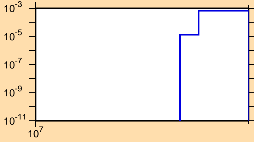
\sigma vs. E for ^{42}\text{K}(n,2np)
