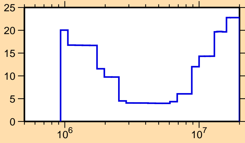
\Delta\sigma/\sigma vs. E for ^{42}\text{K}(n,\text{inel.})
