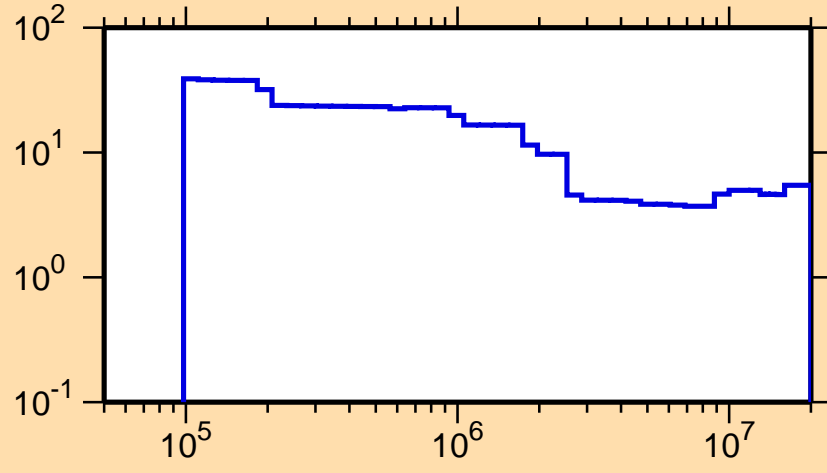
\Delta\sigma/\sigma vs. E for ^{42}\text{K}(n,\text{nonel.})
