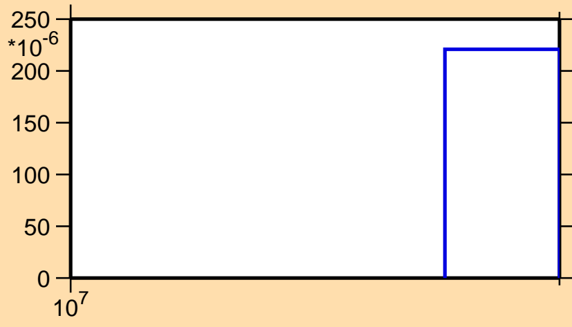
\sigma vs. E for ^{42}\text{K}(n,3n)
