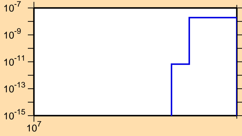
\sigma vs. E for ^{42}\text{K}(n,\text{He}3)
