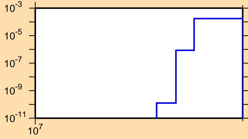
\sigma vs. E for ^{42}\text{K}(n,2n\alpha)
