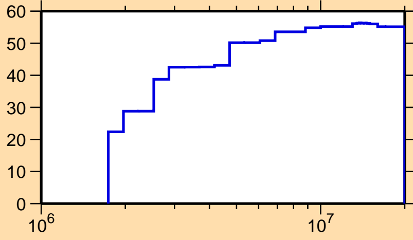
\Delta\sigma/\sigma vs. E for ^{42}\text{K}(n,n_1)
