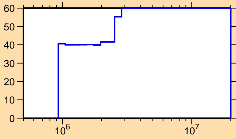
\Delta\sigma/\sigma vs. E for ^{42}\text{K}(n,\gamma)
