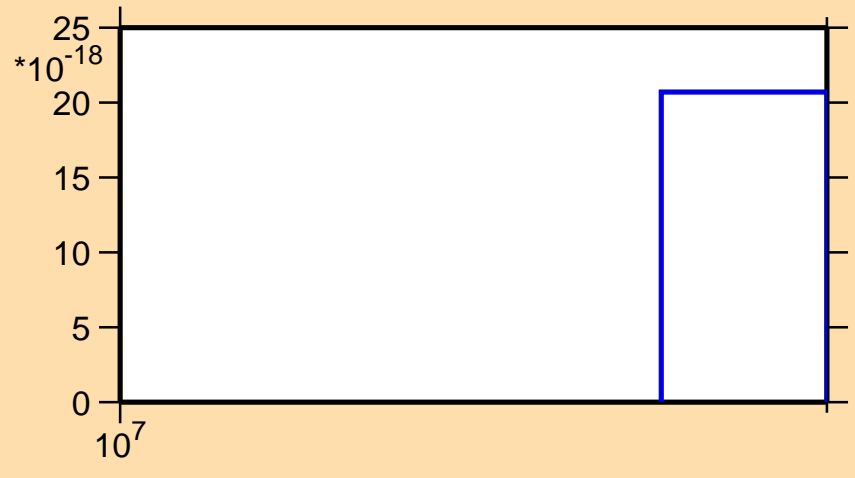
\sigma vs. E for ^{42}\text{K} (mt 45)
