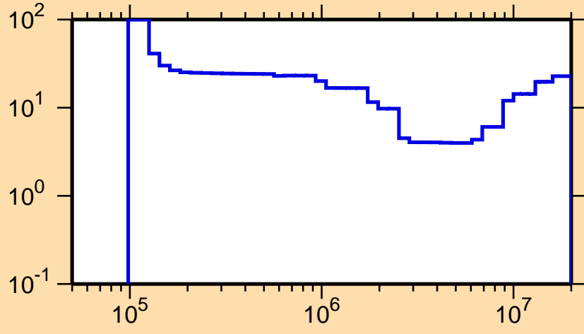
\Delta\sigma/\sigma vs. E for ^{42}\text{K}(n,\text{inel.})
