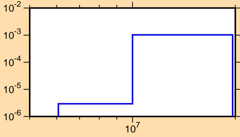
\sigma vs. E for ^{42}\text{K}(n,t)
