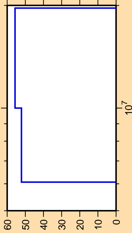
\Delta\sigma/\sigma vs. E for ^{42}\text{K}(n,n_1)
