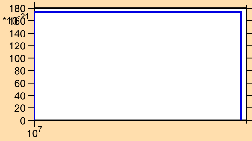
\sigma vs. E for ^{42}\text{K} (mt 45)
