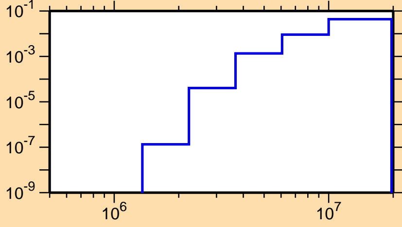
\sigma vs. E for ^{42}\text{K}(n,\alpha)
