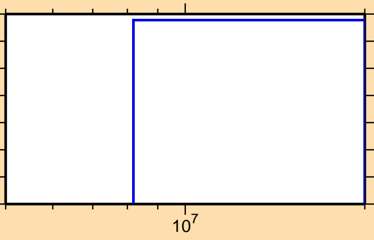
\sigma vs. E for ^{42}\text{K}(n,nd)
