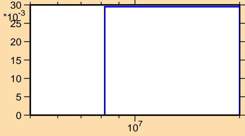
\sigma vs. E for ^{42}\text{K}(n,np)
