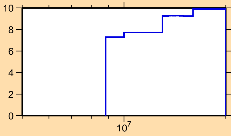
\Delta\sigma/\sigma vs. E for ^{43}\text{K}(n,\text{nonel.})
