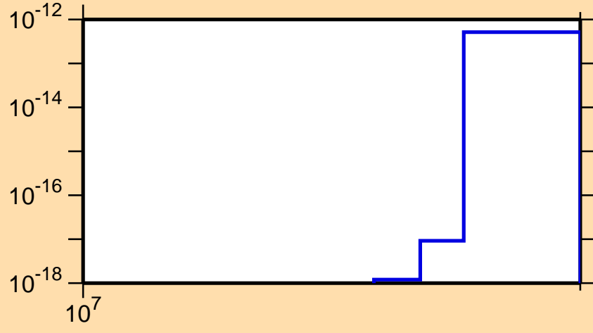
\sigma vs. E for ^{43}\text{K}(n,p\alpha)
