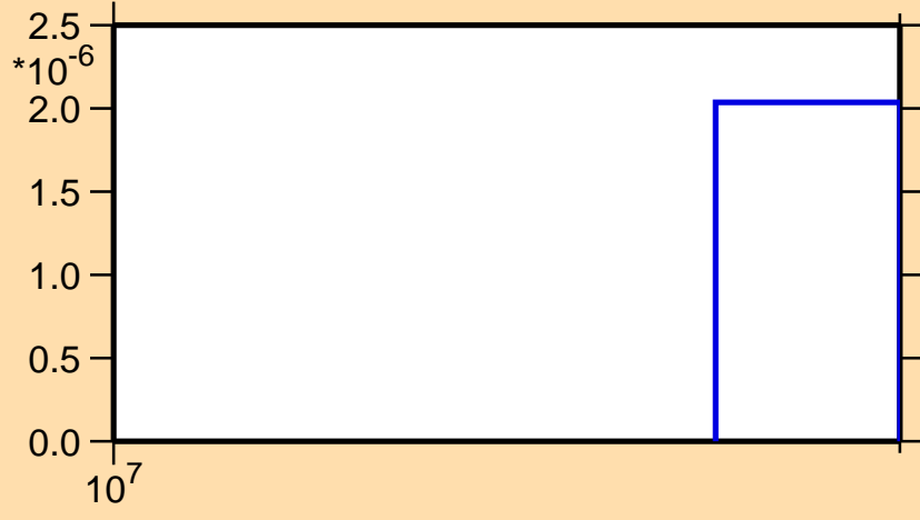
\sigma vs. E for ^{43}\text{K}(n,nd)
