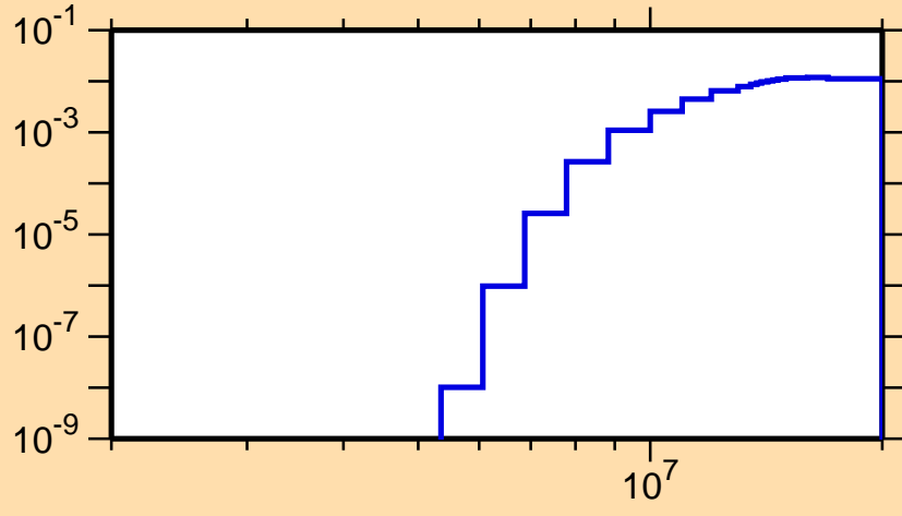
\sigma vs. E for ^{43}\text{K}(n,\alpha)
