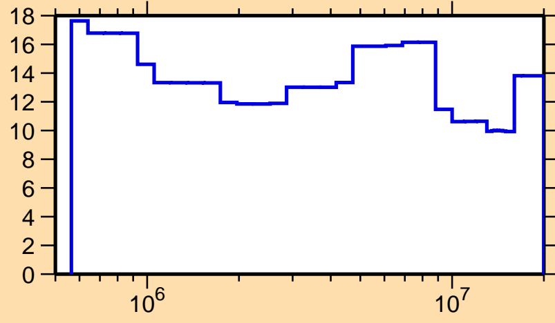
\Delta\sigma/\sigma vs. E for ^{43}\text{K}(n,\text{el.})
