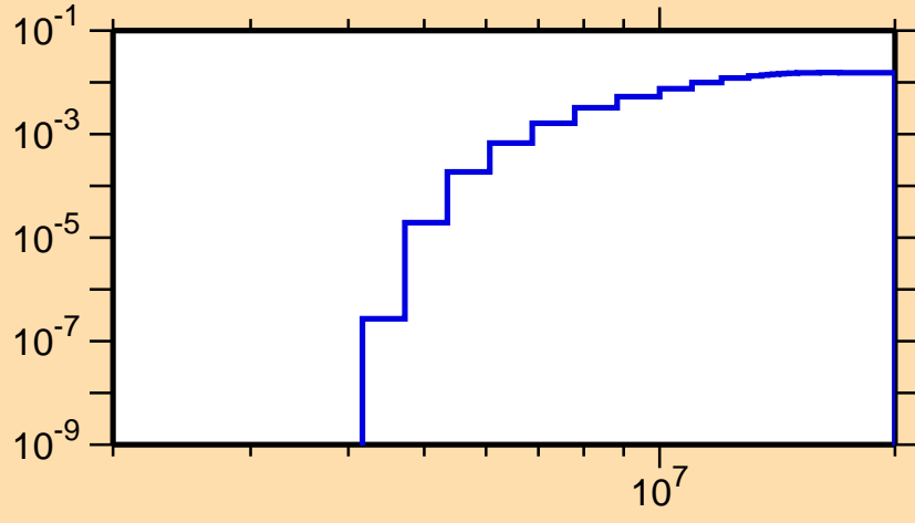
\sigma vs. E for ^{43}\text{K}(n,p)
