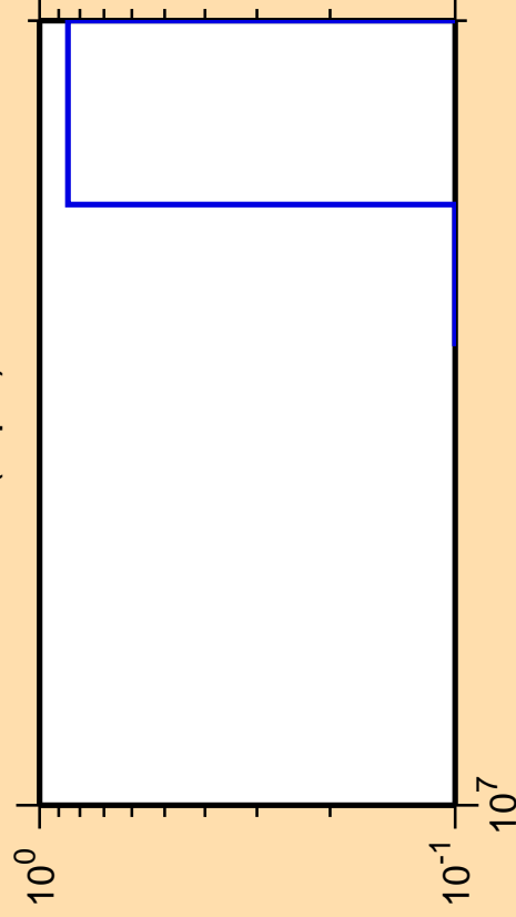
\Delta\sigma/\sigma vs. E for ^{43}\text{K}(n,p\alpha)
