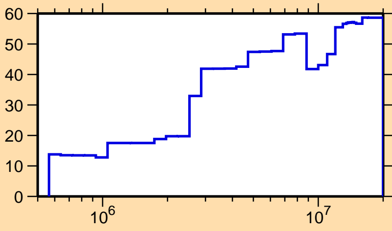
\Delta\sigma/\sigma vs. E for ^{43}\text{K}(n,n_1)
