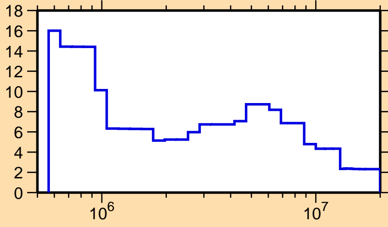
\Delta\sigma/\sigma vs. E for ^{43}\text{K}(n,\text{tot.})
