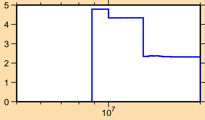
\Delta\sigma/\sigma vs. E for ^{43}\text{K}(n,\text{tot.})
