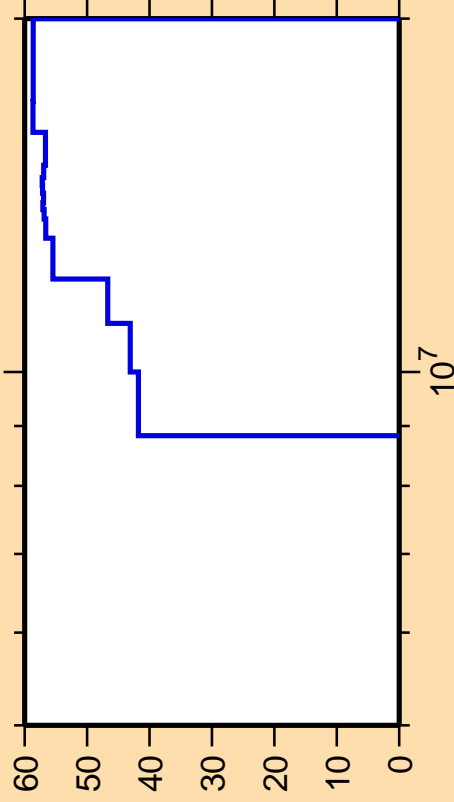
\Delta\sigma/\sigma vs. E for ^{43}\text{K}(n,n_1)
