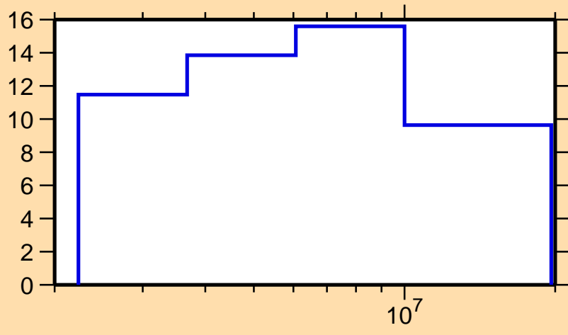
\Delta\sigma/\sigma vs. E for ^{43}\text{K}(n,el.)
