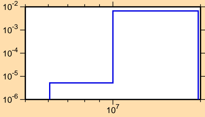
\sigma vs. E for ^{43}\text{K}(n,d)
