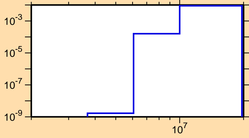
\sigma vs. E for ^{43}\text{K}(n,\alpha)
