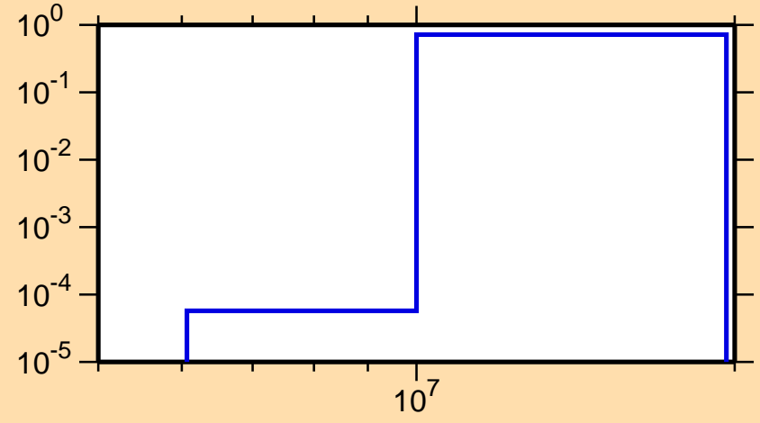
\sigma vs. E for ^{43}\text{K}(n,2n)
