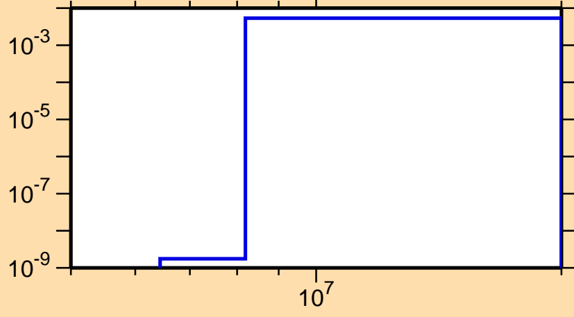
\sigma vs. E for ^{43}\text{K}(n,d)
