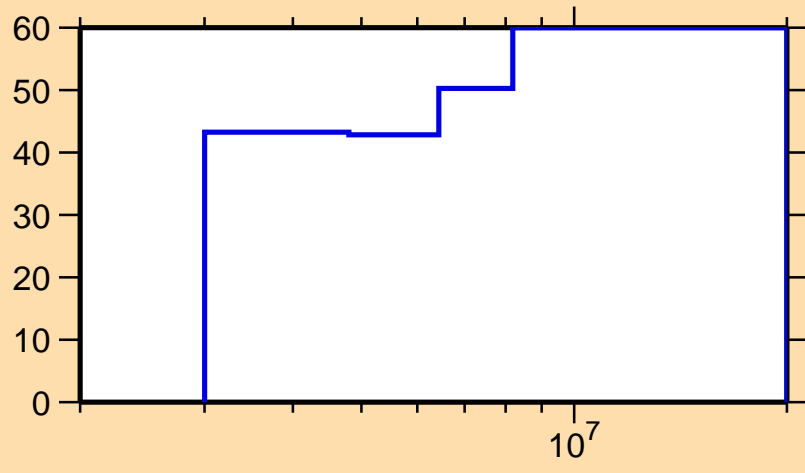
\Delta\sigma/\sigma vs. E for ^{43}\text{K}(n,p)
