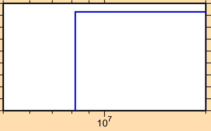
\sigma vs. E for ^{43}\text{K}(n,nd)
