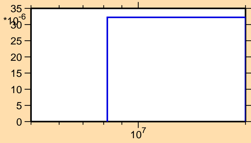
\sigma vs. E for ^{43}\text{K}(n,t)
