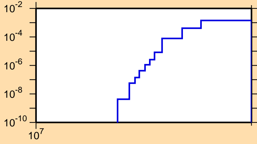
\sigma vs. E for ^{44}\text{K}(n,n\alpha)
