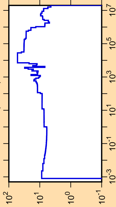
\Delta\sigma/\sigma vs. E for ^{44}\text{K}(n,\text{tot.})
