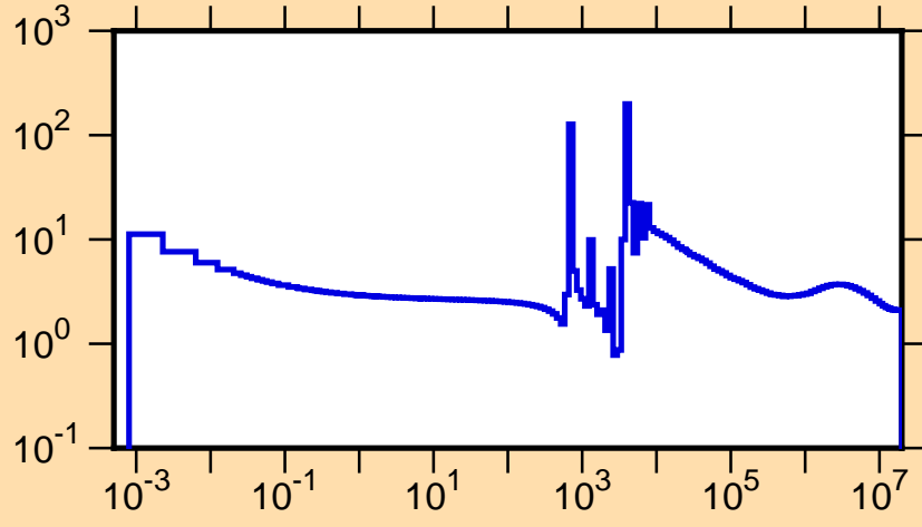
\sigma vs. E for ^{44}\text{K}(n,\text{tot.})
