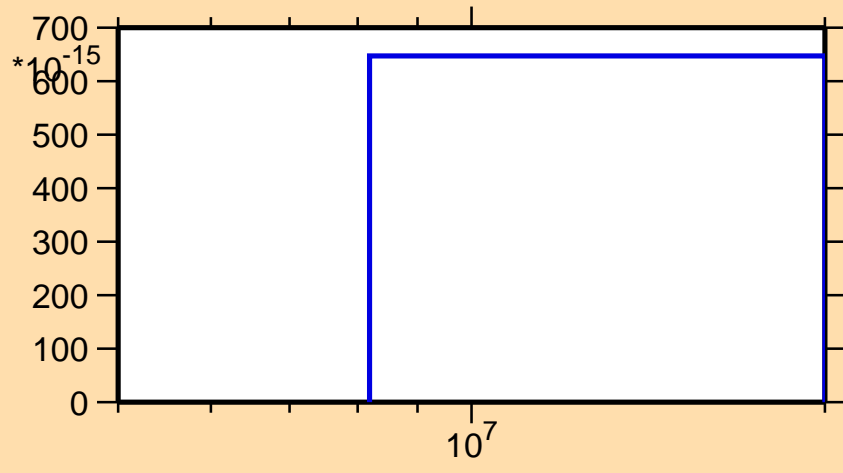
\sigma vs. E for ^{44}\text{K}(n,2n\alpha)
