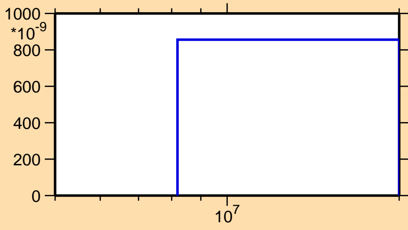
\sigma vs. E for ^{44}\text{K}(n,nd)
