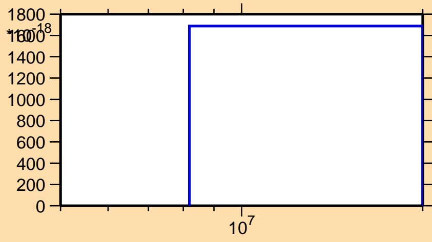
\sigma vs. E for ^{44}\text{K}(n,p\alpha)
