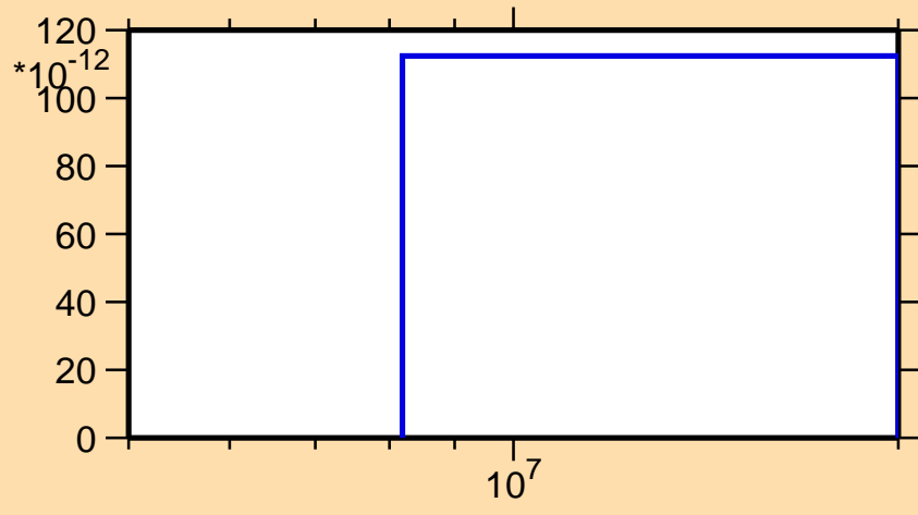
\sigma vs. E for ^{44}\text{K}(n,nt)
