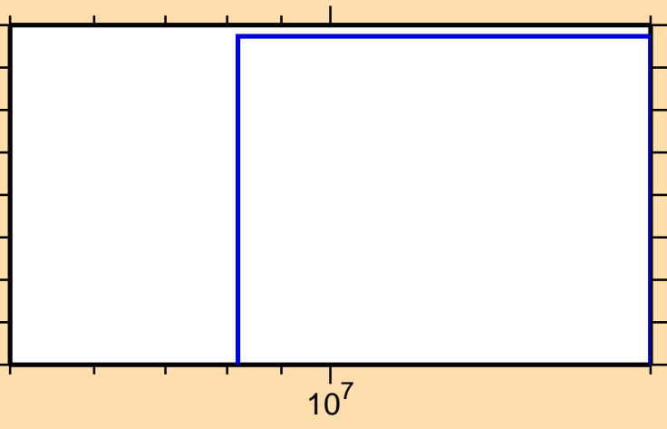
\sigma vs. E for ^{44}\text{K}(n,np)
