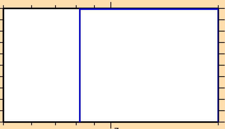
\sigma vs. E for ^{44}\text{K}(n,3n)
