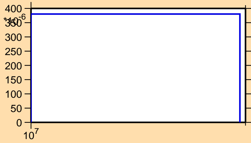
\sigma vs. E for ^{46}\text{K}(n,d)
