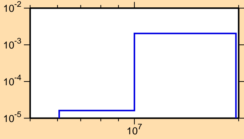
\sigma vs. E for ^{46}\text{K}(n,\alpha)
