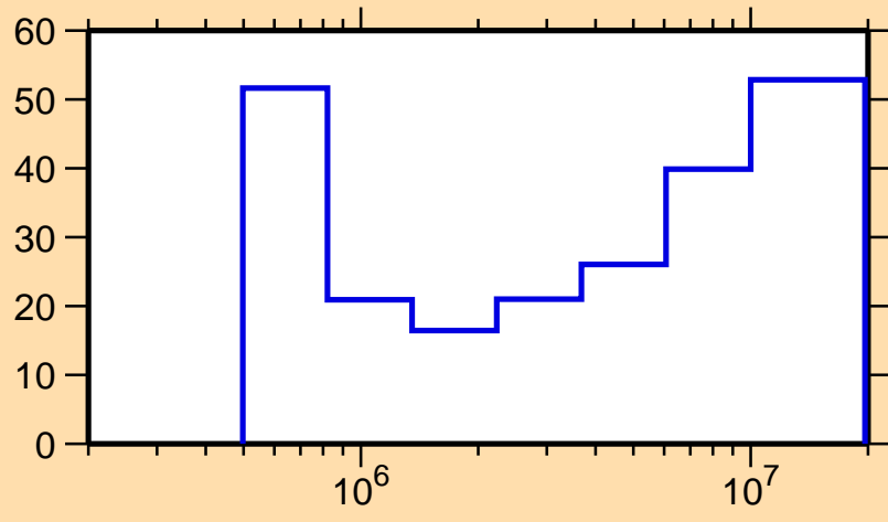
\Delta\sigma/\sigma vs. E for ^{46}\text{K}(n,\text{el.})
