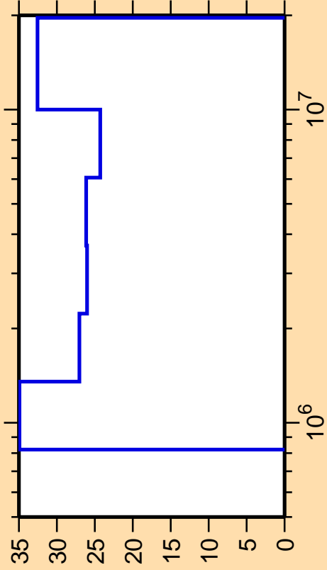
\Delta\sigma/\sigma vs. E for ^{46}\text{K}(n,n_3)
