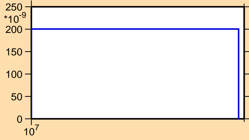
\sigma vs. E for ^{46}\text{K}(n,n\alpha)
