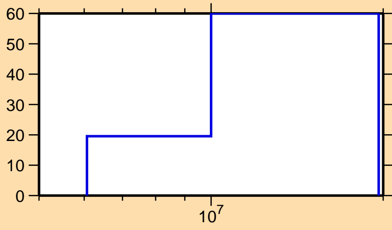
\Delta\sigma/\sigma vs. E for ^{46}\text{K}(n,\text{inel.})
