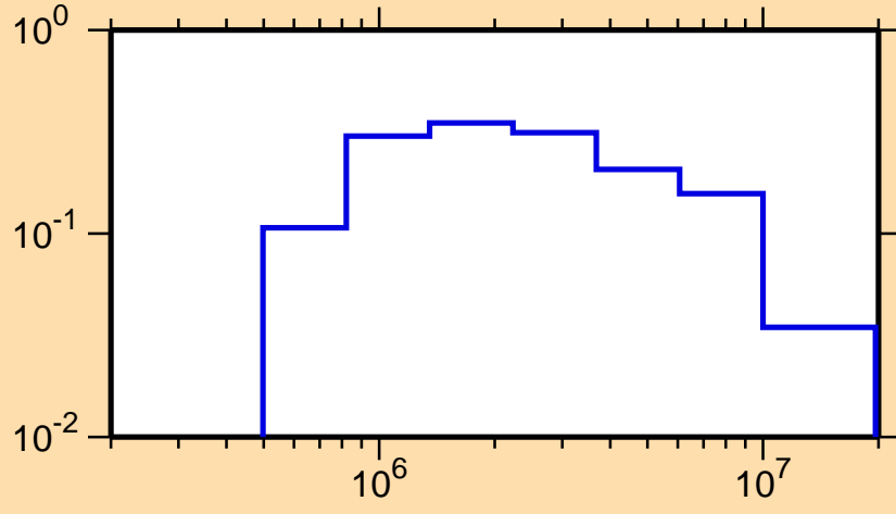
\sigma vs. E for ^{46}\text{K}(n,n_1)
