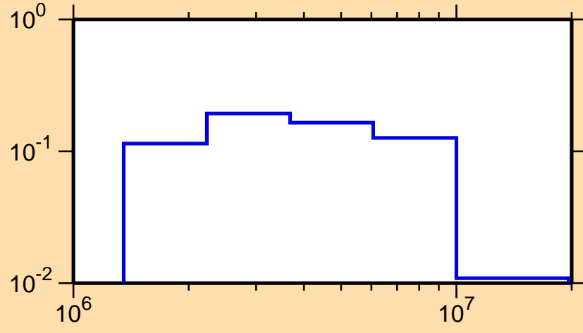
\sigma vs. E for ^{46}\text{K}(n,n_4)
