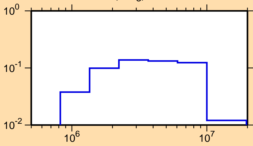
\sigma vs. E for ^{46}\text{K}(n,n_3)
