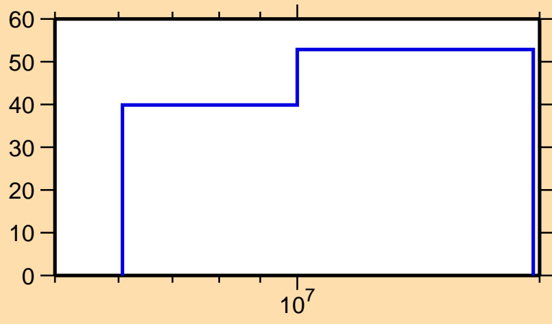
\Delta\sigma/\sigma vs. E for ^{46}\text{K}(n,el.)
