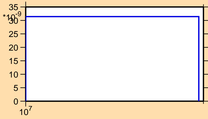
\sigma vs. E for ^{46}\text{K}(n,nd)
