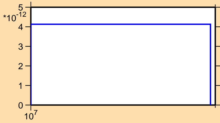
\sigma vs. E for ^{46}\text{K}(n,2np)
