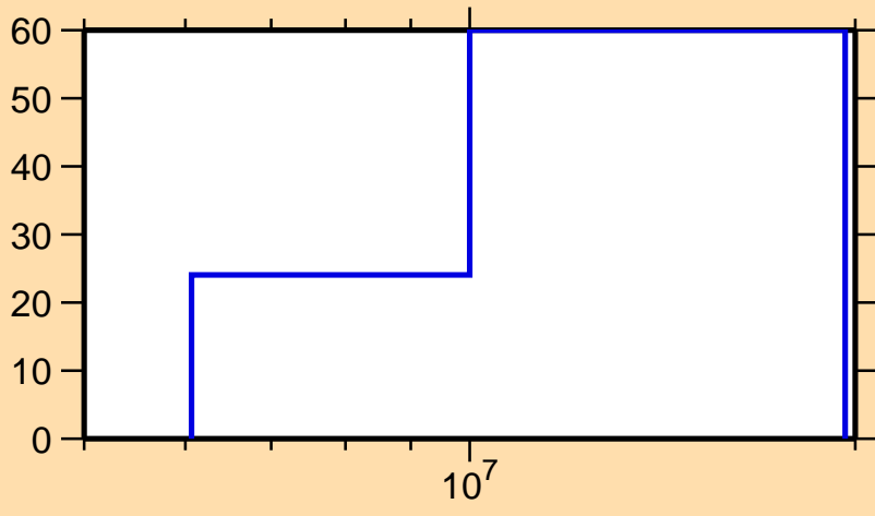
\Delta\sigma/\sigma vs. E for ^{46}\text{K}(n,n_1)
