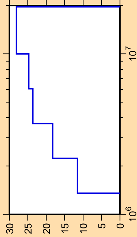
\Delta\sigma/\sigma vs. E for ^{46}\text{K}(n,n_4)
