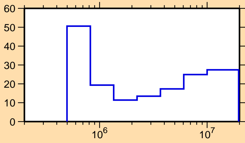
\Delta\sigma/\sigma vs. E for ^{46}\text{K}(n,\text{tot.})
