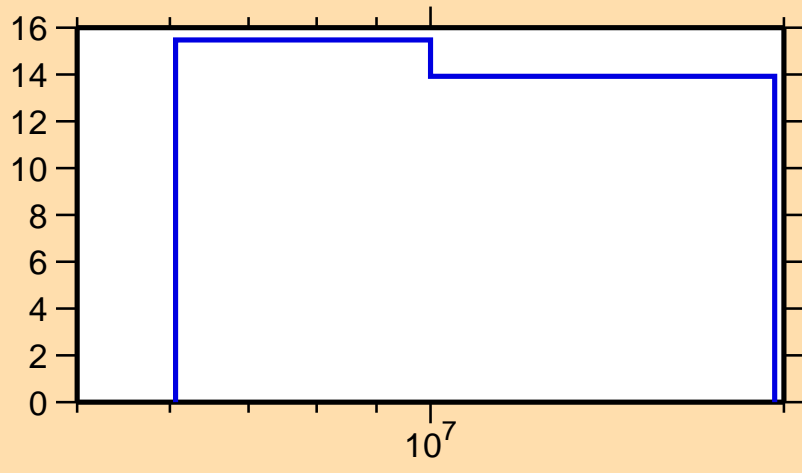
\Delta\sigma/\sigma vs. E for ^{46}\text{K}(n,\text{nonel.})
