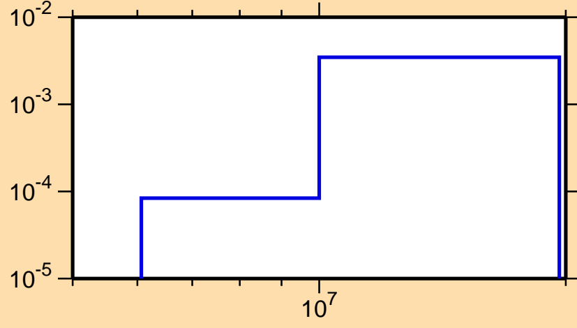
\sigma vs. E for ^{46}\text{K}(n,n\text{cont.})
