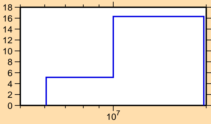
\Delta\sigma/\sigma vs. E for ^{46}\text{K}(n,2n)
