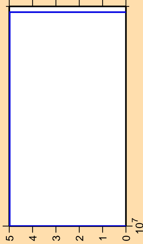
\Delta\sigma/\sigma vs. E for ^{46}\text{K}(n,nt)
