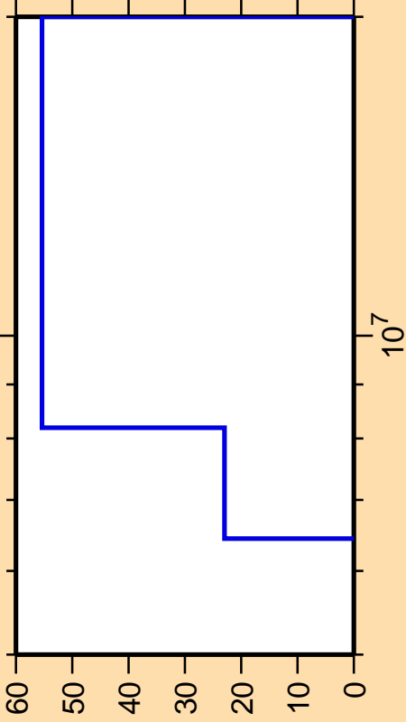
\Delta\sigma/\sigma vs. E for ^{46}\text{K}(n,\alpha)
