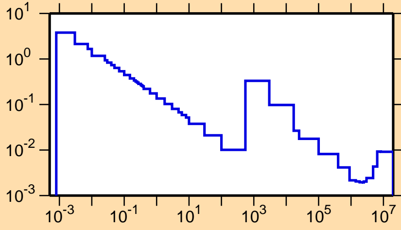
\sigma vs. E for ^{46}\text{K}(n,\gamma)
