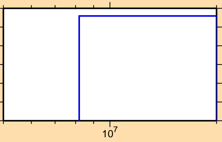
\sigma vs. E for ^{46}\text{K}(n,np)
