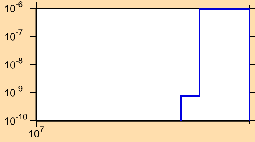
\sigma vs. E for ^{47}\text{K}(n,n\alpha)
