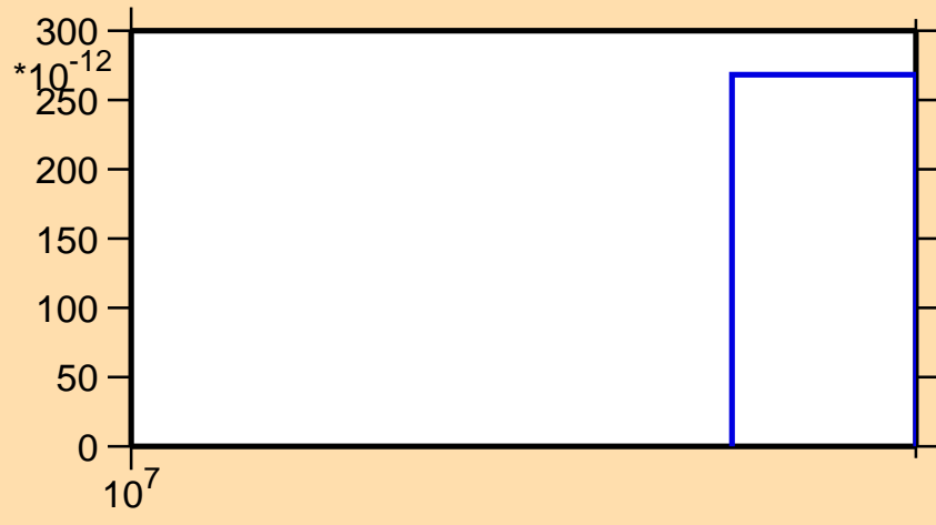
\sigma vs. E for ^{47}\text{K}(n,nt)
