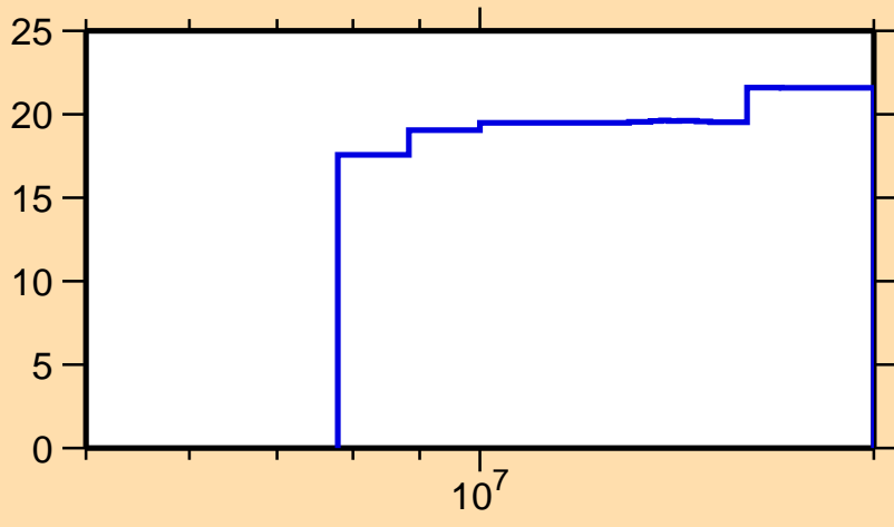
\Delta\sigma/\sigma vs. E for ^{47}\text{K}(n,n\text{onel.})
