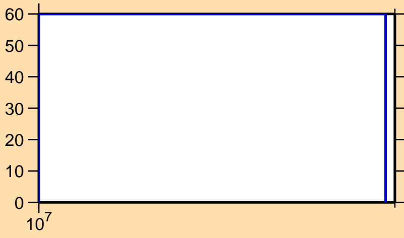
\Delta\sigma/\sigma vs. E for ^{47}\text{K}(n,p)
