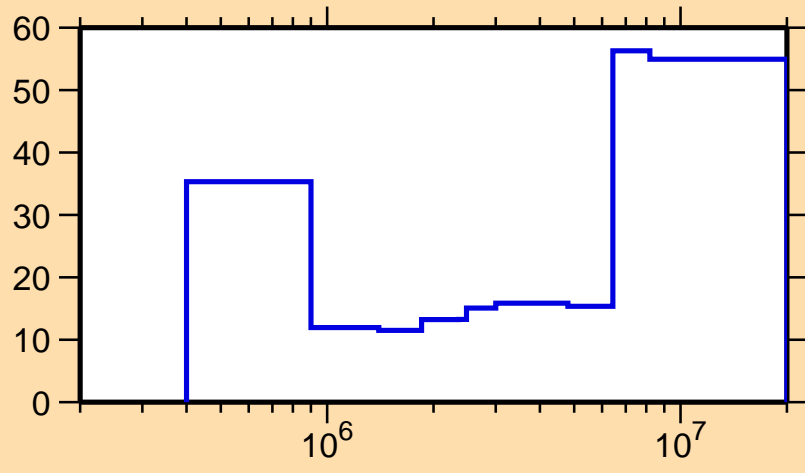
\Delta\sigma/\sigma vs. E for ^{47}\text{K}(n,n_1)
