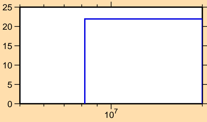
\Delta\sigma/\sigma vs. E for ^{47}\text{K}(n,2n)
