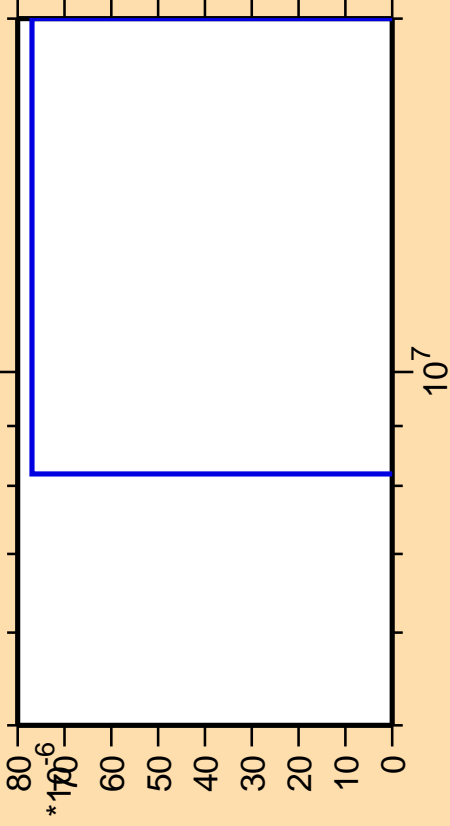
\Delta\sigma/\sigma vs. E for ^{47}\text{K}(n,nd)
