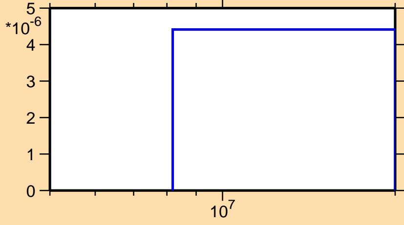
\sigma vs. E for ^{47}\text{K}(n,\alpha)
