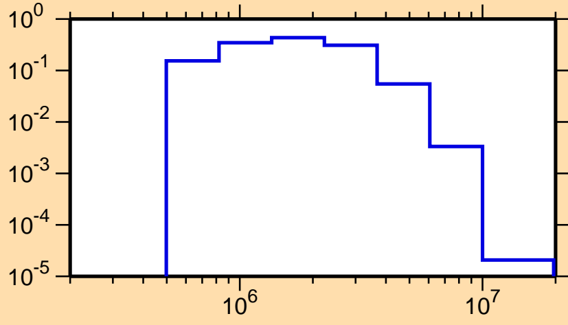
\sigma vs. E for ^{48}\text{K}(n,n_2)
