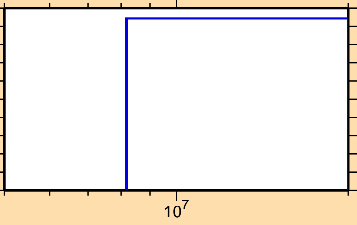
\sigma vs. E for ^{48}\text{K}(n,3n)
