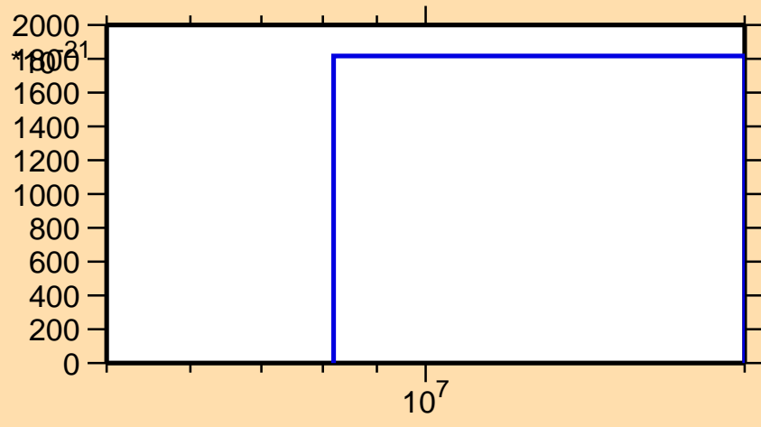
\sigma vs. E for ^{48}\text{K}(n,2n\alpha)
