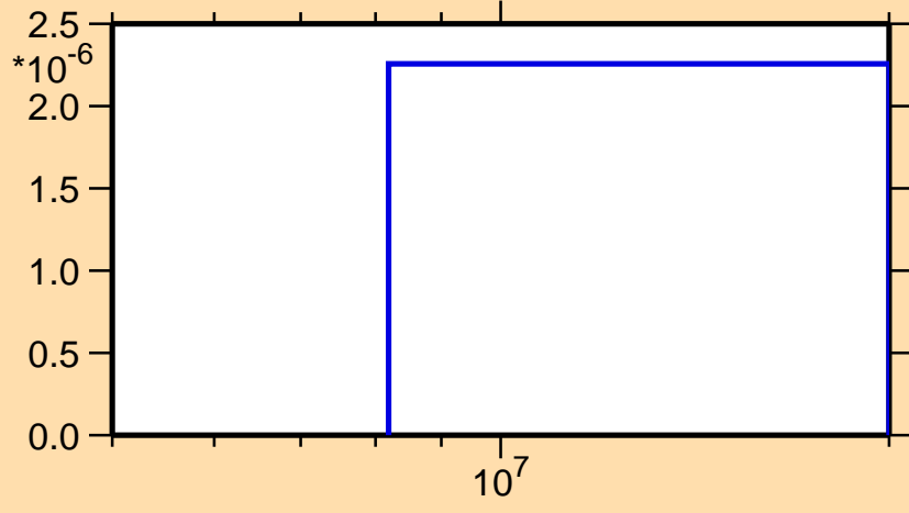
\sigma vs. E for ^{48}\text{K}(n,\alpha)
