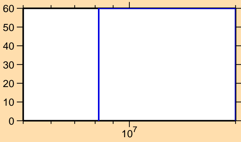
\Delta\sigma/\sigma vs. E for ^{48}\text{K}(n,\gamma)
