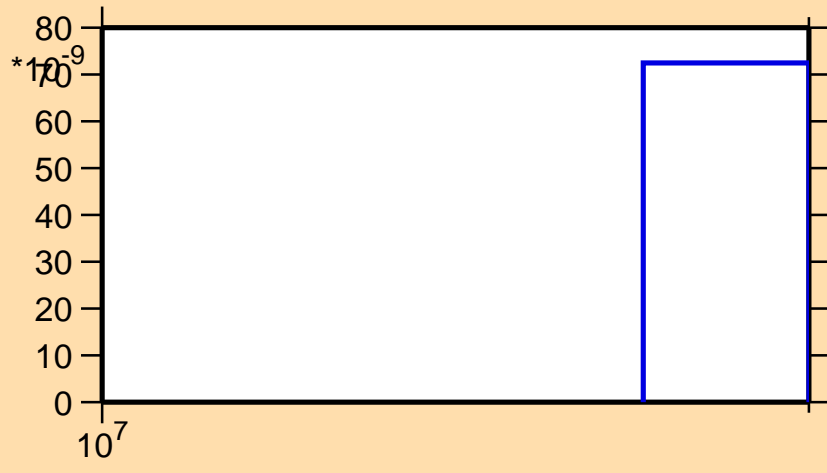
\sigma vs. E for ^{49}\text{K}(n,\text{nd})
