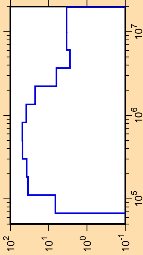
\Delta\mu/\mu vs. E for ^{49}\text{K}(\text{mt251})
