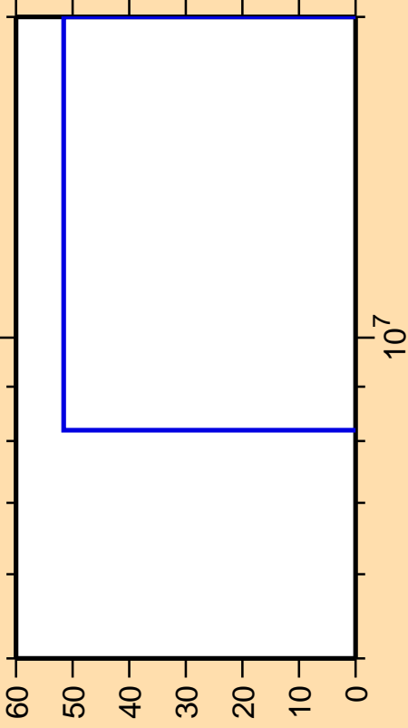
\Delta\sigma/\sigma vs. E for ^{49}\text{K}(n,d)
