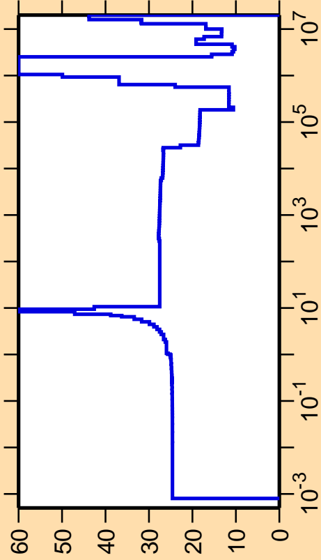
\Delta\sigma/\sigma vs. E for ^{72}\text{Kr}(n,\text{el.})
