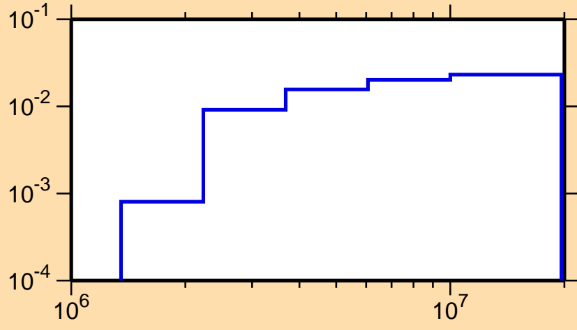
\sigma vs. E for ^{72}\text{Kr}(n,n_4)
