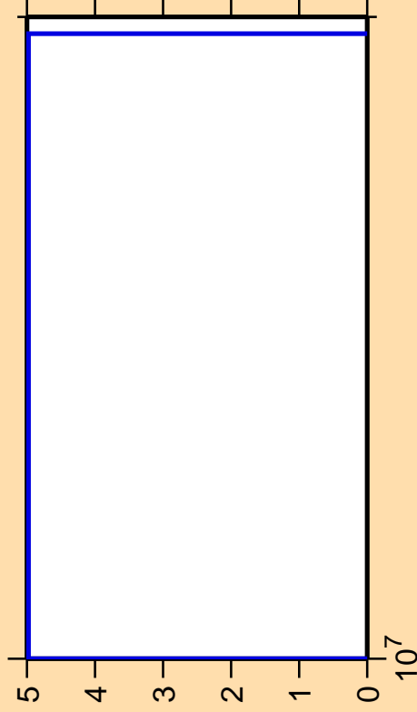
\Delta\sigma/\sigma vs. E for ^{72}\text{Kr}(n,nd)
