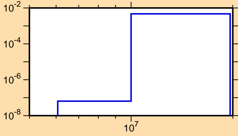
\sigma vs. E for ^{72}\text{Kr}(n,pd)
