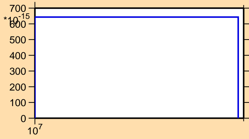
\sigma vs. E for ^{72}\text{Kr}(n,nd)
