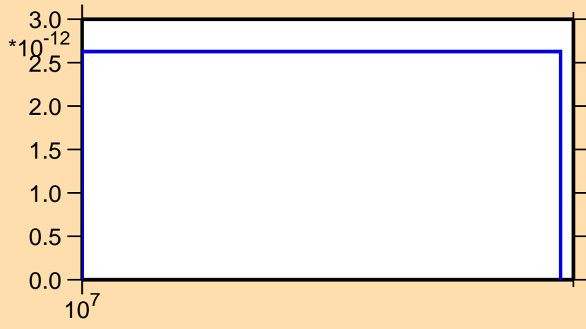
\sigma vs. E for ^{72}\text{Kr}(n,2np)
