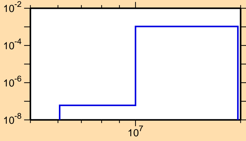
\sigma vs. E for ^{72}\text{Kr}(n,\alpha)
