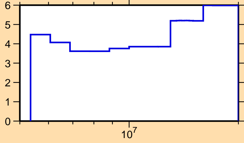
\Delta\sigma/\sigma vs. E for ^{73}\text{Kr}(n,n\text{onel.})
