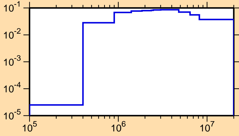
\sigma vs. E for ^{73}\text{Kr}(n,n_2)
