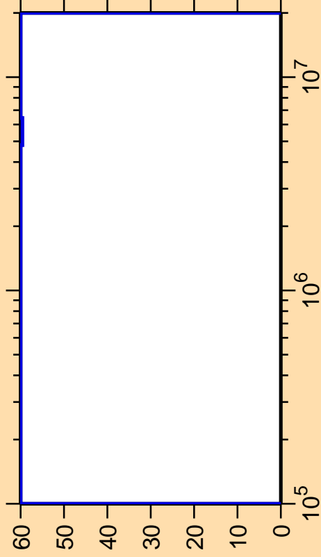
\Delta\sigma/\sigma vs. E for ^{73}\text{Kr}(n,n_2)
