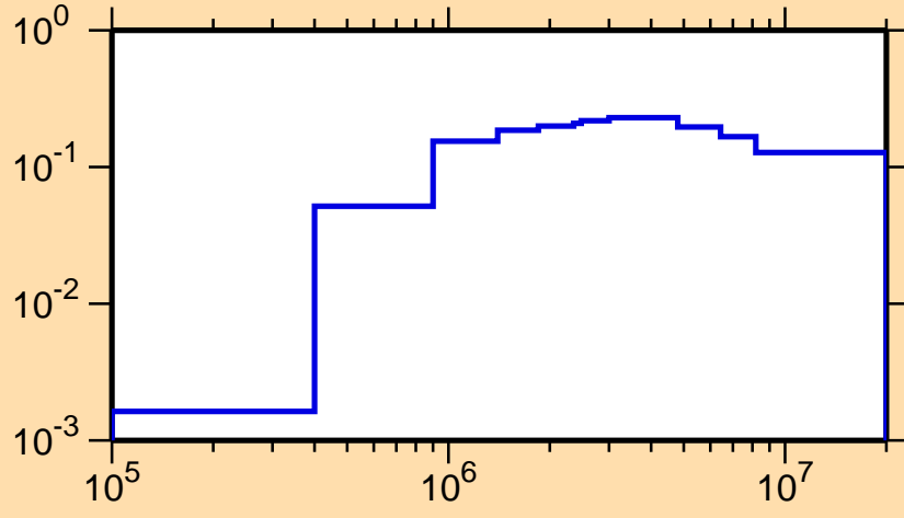
\sigma vs. E for ^{73}\text{Kr}(n,\text{inel.})
