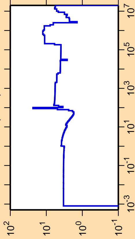
\Delta\sigma/\sigma vs. E for ^{74}\text{Kr}(n,\text{el.})
