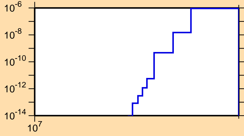
\sigma vs. E for ^{74}\text{Kr}(\text{mt } 45)
