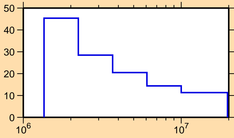
\Delta\sigma/\sigma vs. E for ^{74}\text{Kr}(n,inel.)
