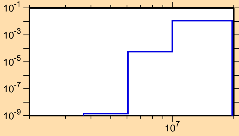
\sigma vs. E for ^{74}\text{Kr}(n,d)
