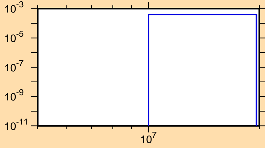
\sigma vs. E for ^{74}\text{Kr}(n,pd)
