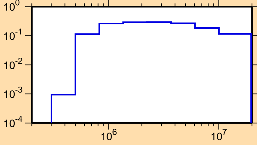
\sigma vs. E for ^{74}\text{Kr}(n,n_1)
